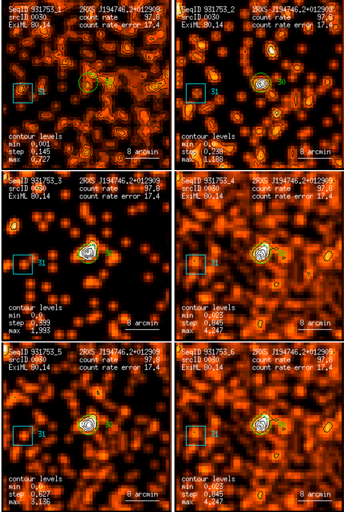
Figure 30: RASS 931753: detection 0030: band rate images, Gaussian filter: (1) PSPC channels 11 – 41, (2) 52 – 90, (3) 91 – 201, (4) 11 – 235, (5) 52 – 201, (6) 11 – 201. Broad band rates in counts/ks. Band rate contour levels in counts/ks/arcmin 2 .
