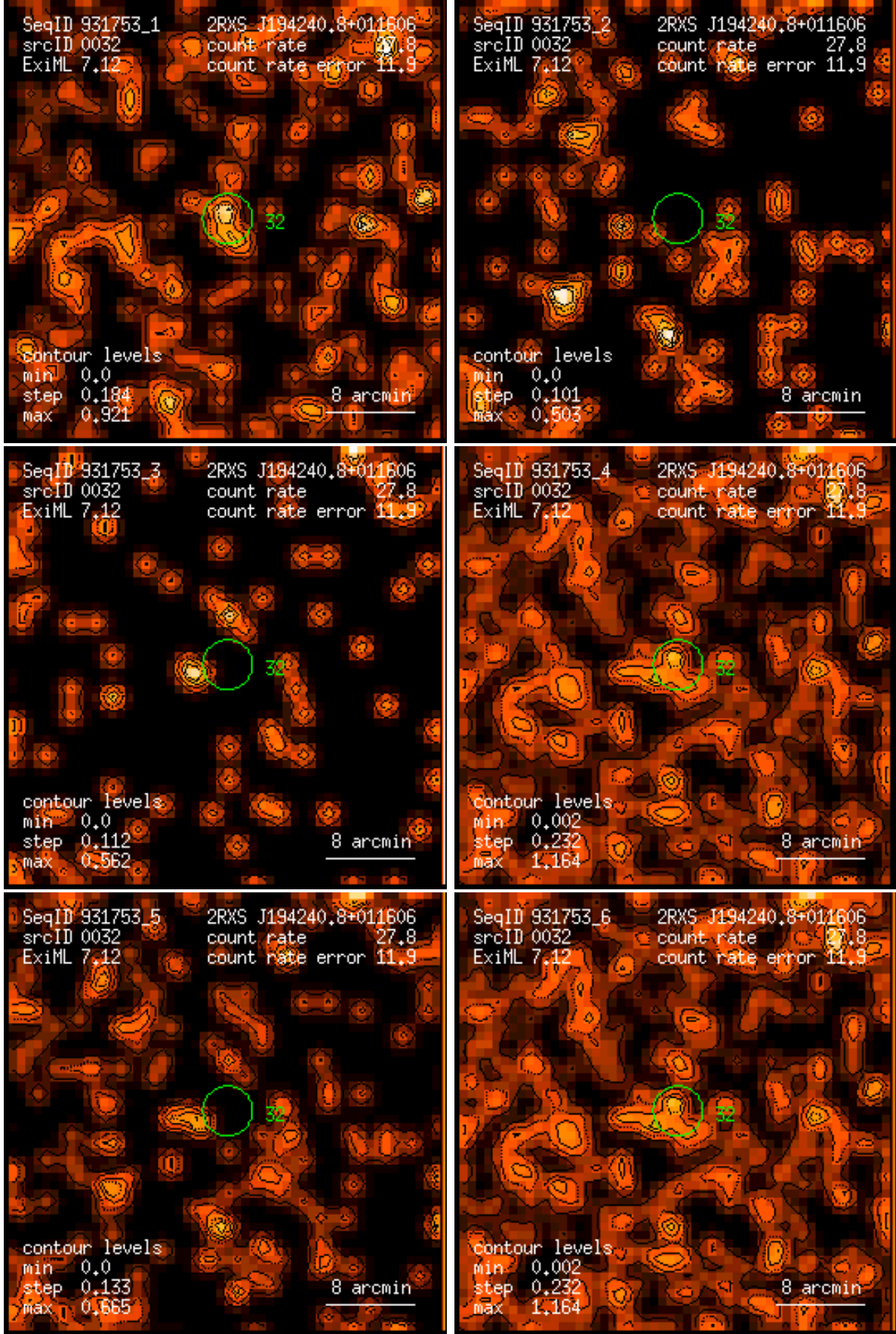
Figure 32: RASS 931753: detection 0032: band rate images, Gaussian filter: (1) PSPC channels 11 – 41, (2) 52 – 90, (3) 91 – 201, (4) 11 – 235, (5) 52 – 201, (6) 11 – 201. Broad band rates in counts/ks. Band rate contour levels in counts/ks/arcmin 2 .
