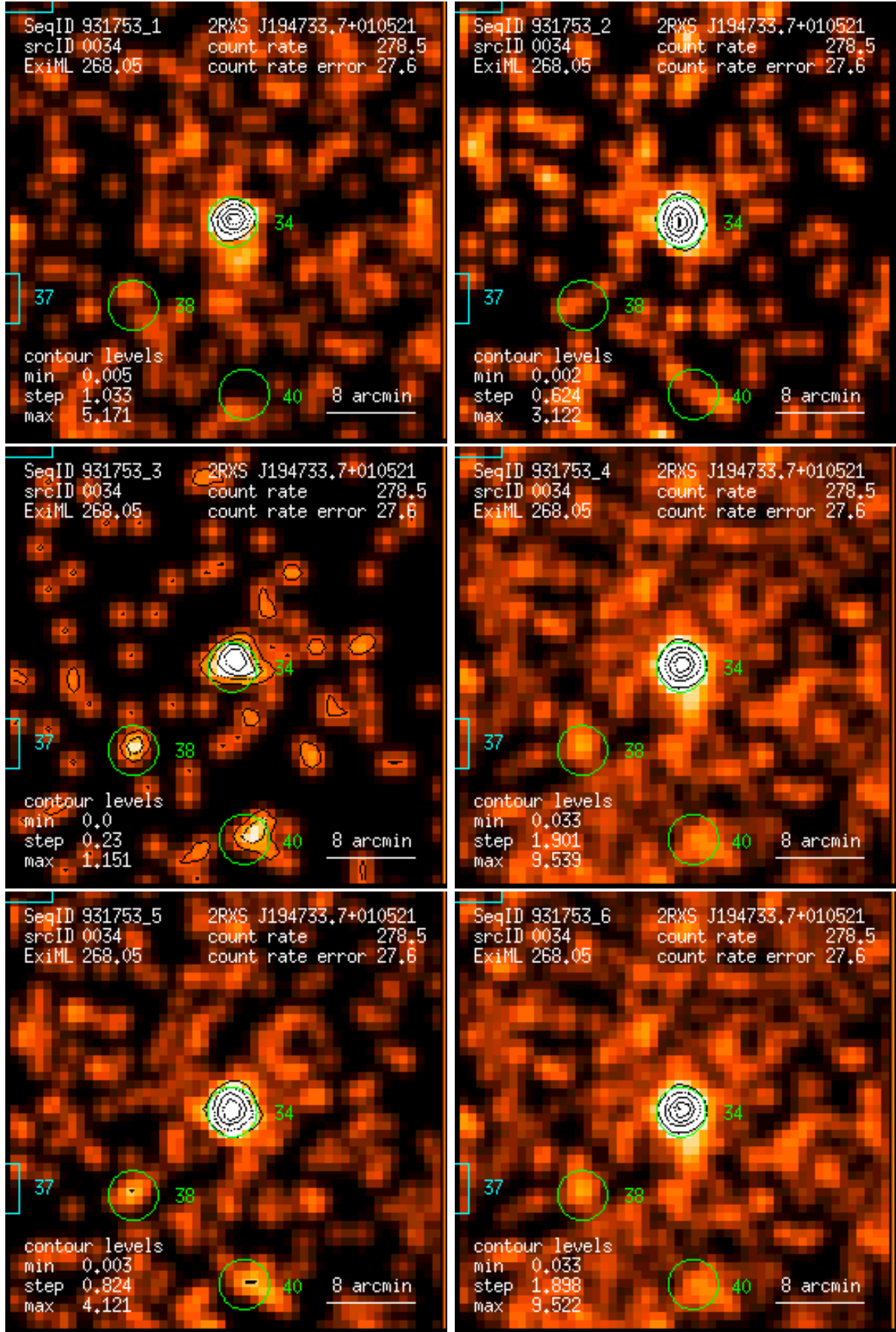
Figure 34: RASS 931753: detection 0034: band rate images, Gaussian filter: (1) PSPC channels 11 – 41, (2) 52 – 90, (3) 91 – 201, (4) 11 – 235, (5) 52 – 201, (6) 11 – 201. Broad band rates in counts/ks. Band rate contour levels in counts/ks/arcmin 2 .
