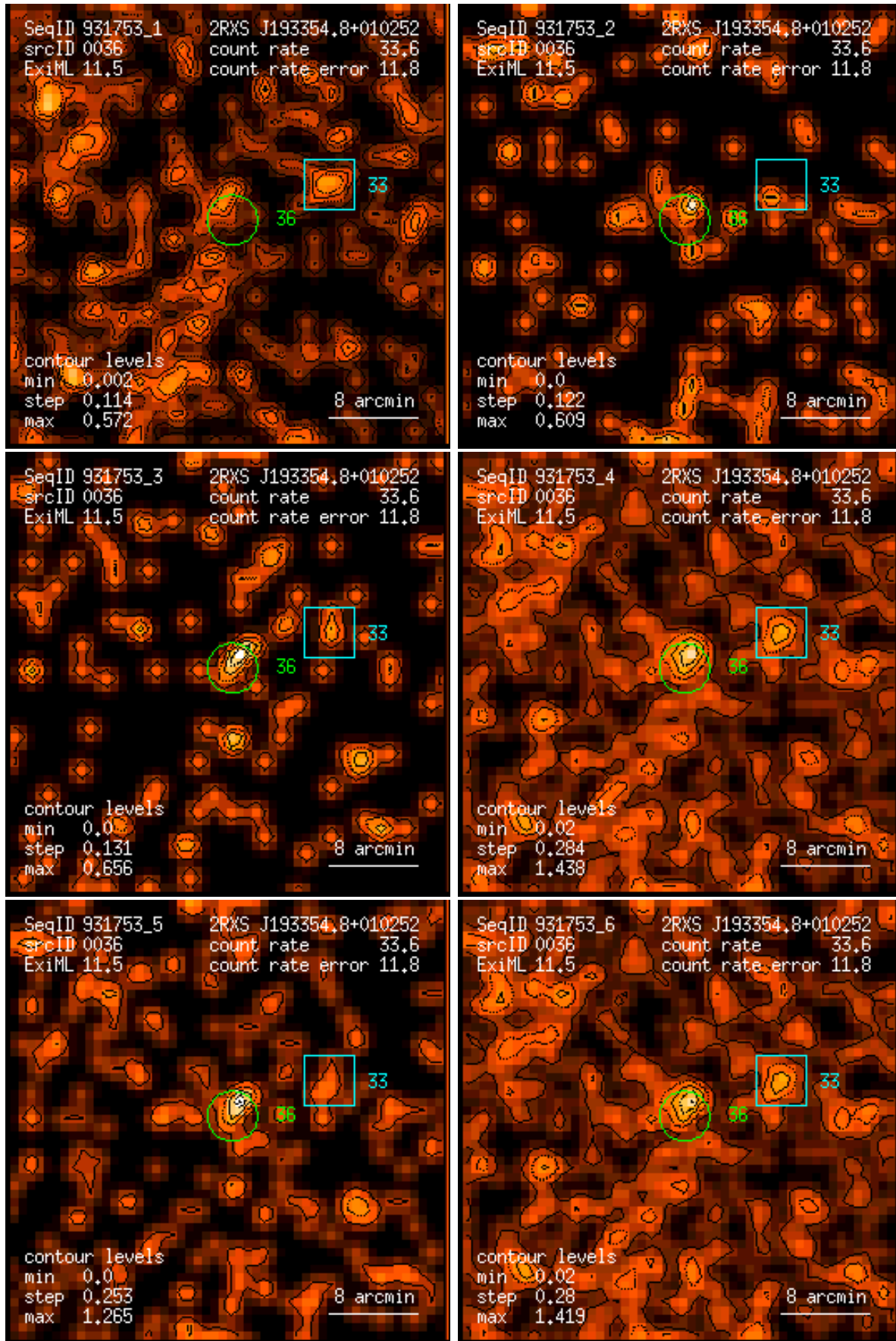
Figure 36: RASS 931753: detection 0036: band rate images, Gaussian filter: (1) PSPC channels 11 – 41, (2) 52 – 90, (3) 91 – 201, (4) 11 – 235, (5) 52 – 201, (6) 11 – 201. Broad band rates in counts/ks. Band rate contour levels in counts/ks/arcmin 2 .
