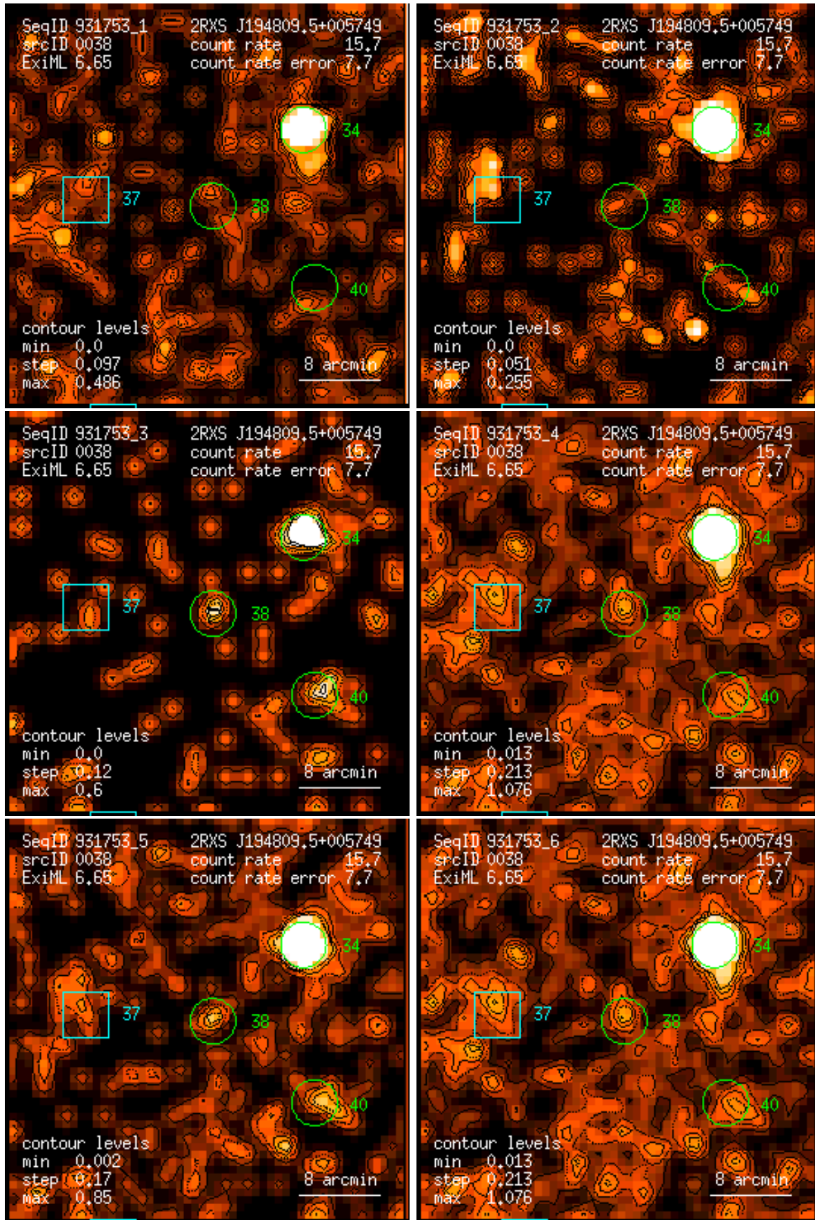
Figure 38: RASS 931753: detection 0038: band rate images, Gaussian filter: (1) PSPC channels 11 – 41, (2) 52 – 90, (3) 91 – 201, (4) 11 – 235, (5) 52 – 201, (6) 11 – 201. Broad band rates in counts/ks. Band rate contour levels in counts/ks/arcmin 2 .
