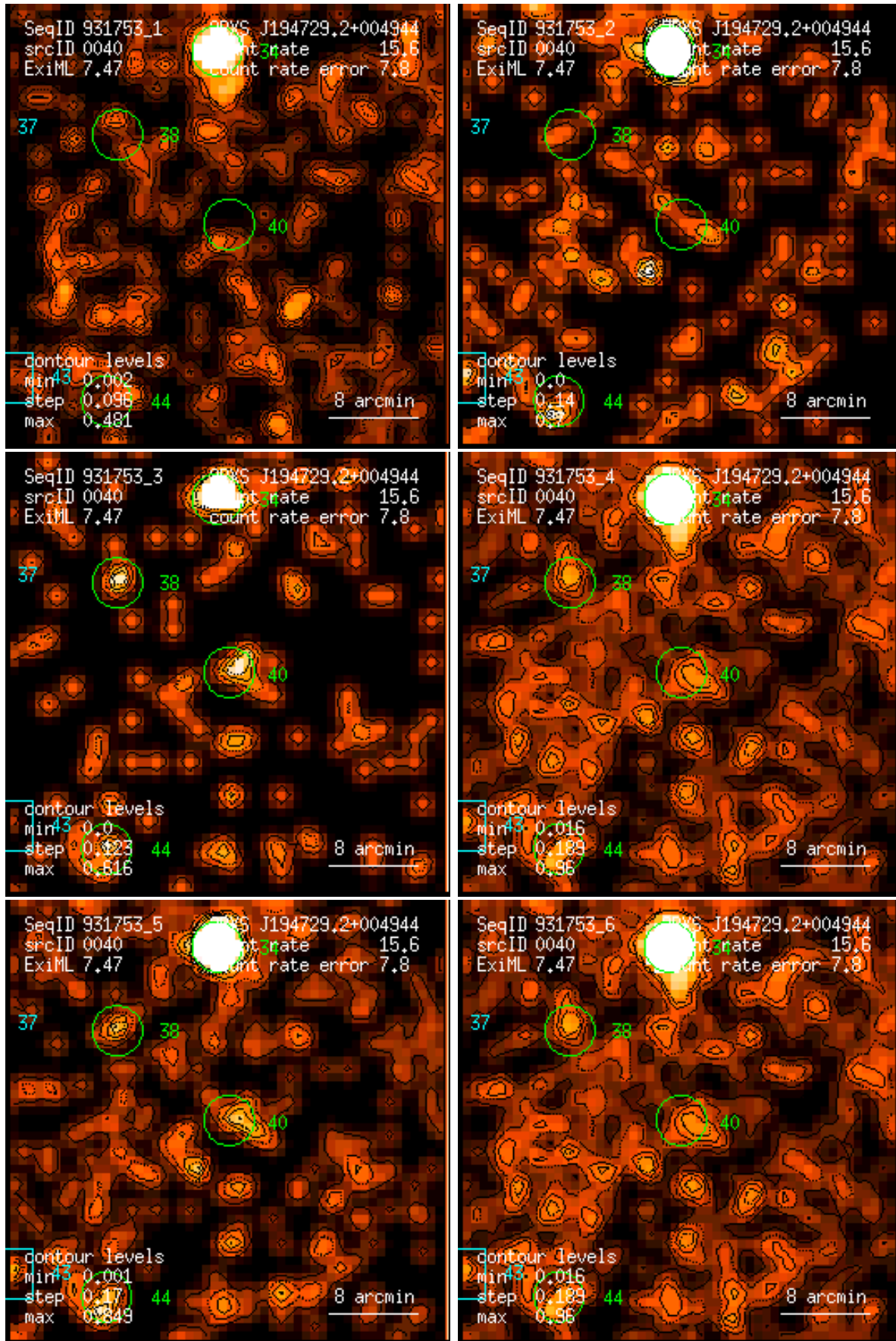
Figure 40: RASS 931753: detection 0040: band rate images, Gaussian filter: (1) PSPC channels 11 – 41, (2) 52 – 90, (3) 91 – 201, (4) 11 – 235, (5) 52 – 201, (6) 11 – 201. Broad band rates in counts/ks. Band rate contour levels in counts/ks/arcmin 2 .
