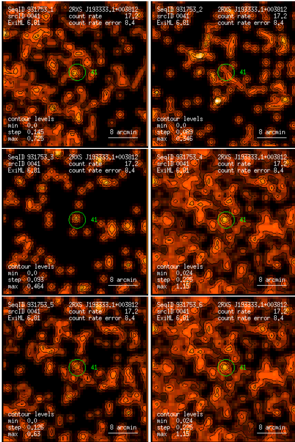
Figure 41: RASS 931753: detection 0041: band rate images, Gaussian filter: (1) PSPC channels 11 – 41, (2) 52 – 90, (3) 91 – 201, (4) 11 – 235, (5) 52 – 201, (6) 11 – 201. Broad band rates in counts/ks. Band rate contour levels in counts/ks/arcmin 2 .
