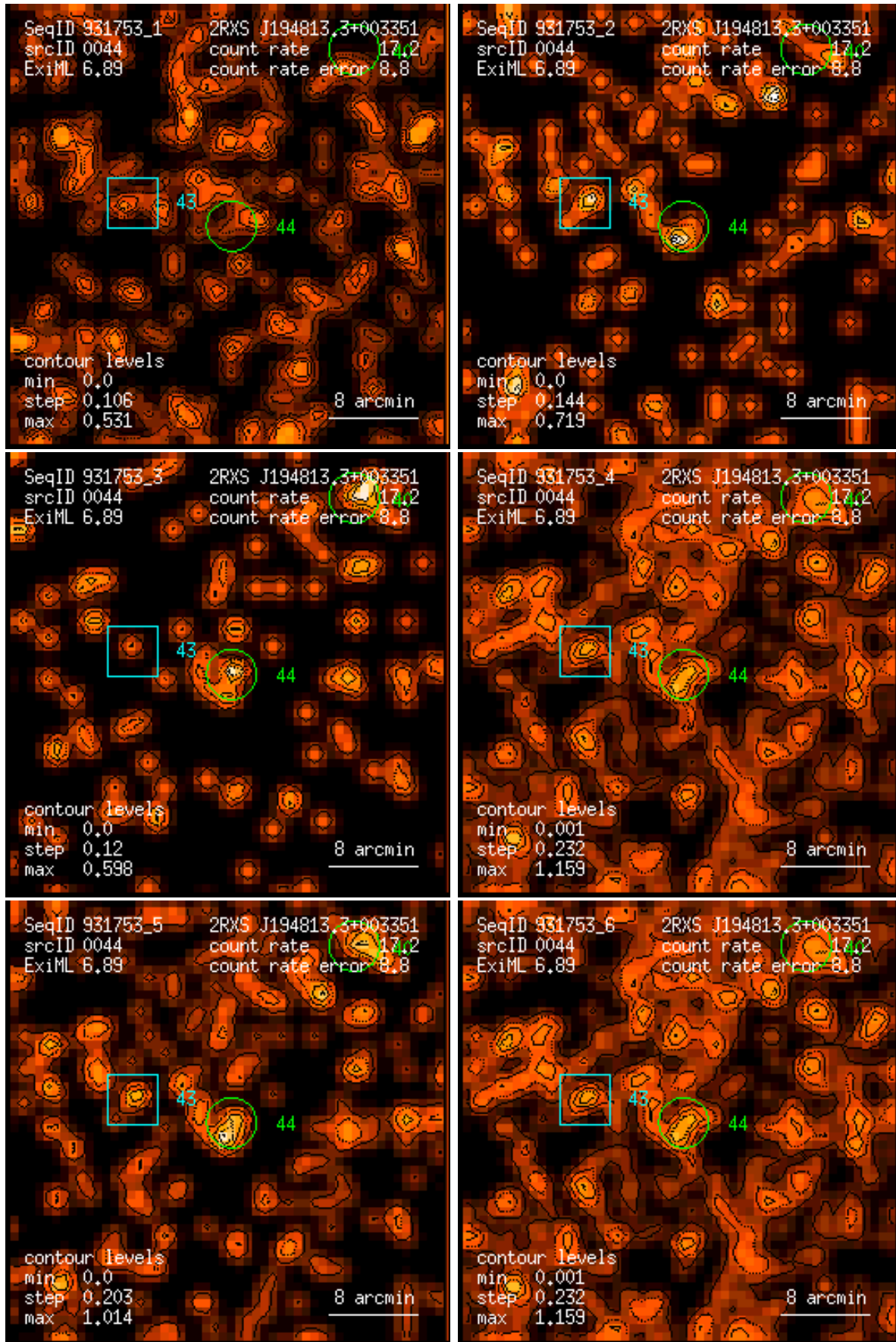
Figure 44: RASS 931753: detection 0044: band rate images, Gaussian filter: (1) PSPC channels 11 – 41, (2) 52 – 90, (3) 91 – 201, (4) 11 – 235, (5) 52 – 201, (6) 11 – 201. Broad band rates in counts/ks. Band rate contour levels in counts/ks/arcmin 2 .
