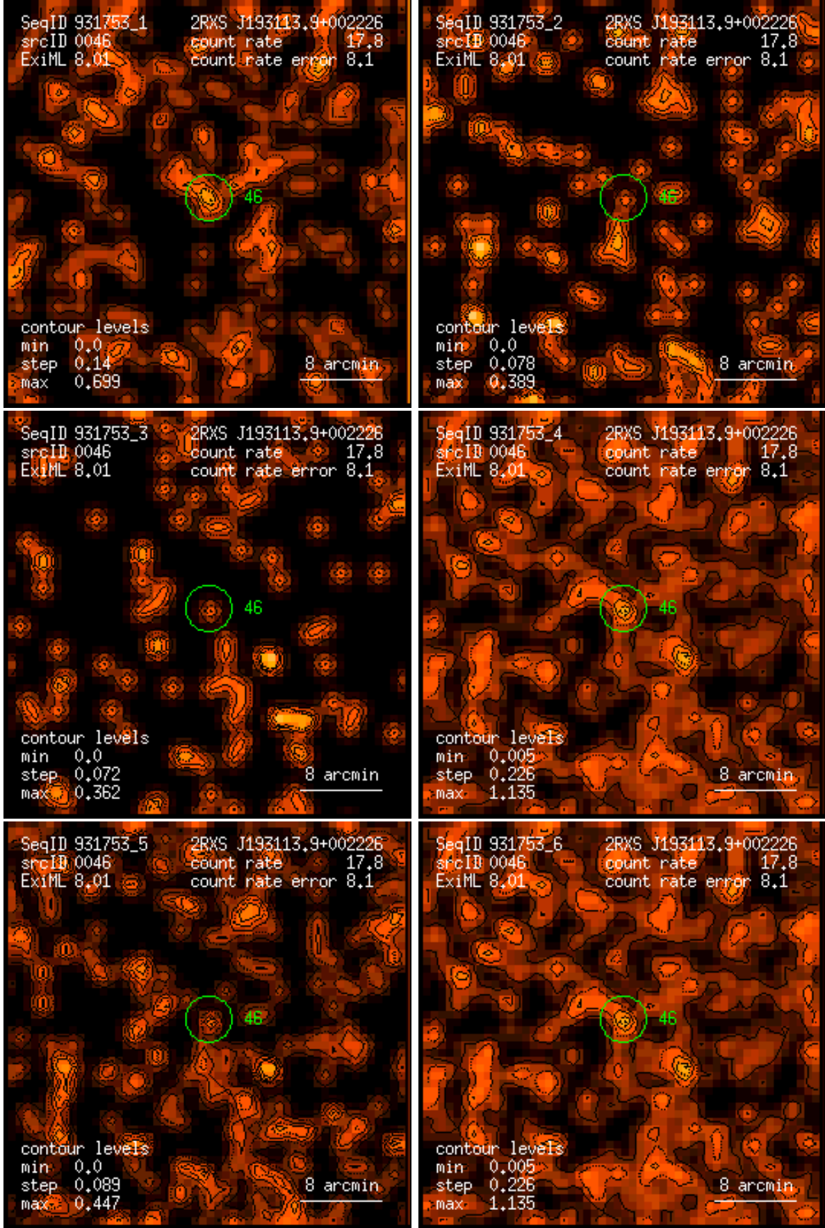
Figure 46: RASS 931753: detection 0046: band rate images, Gaussian filter: (1) PSPC channels 11 – 41, (2) 52 – 90, (3) 91 – 201, (4) 11 – 235, (5) 52 – 201, (6) 11 – 201. Broad band rates in counts/ks. Band rate contour levels in counts/ks/arcmin 2 .
