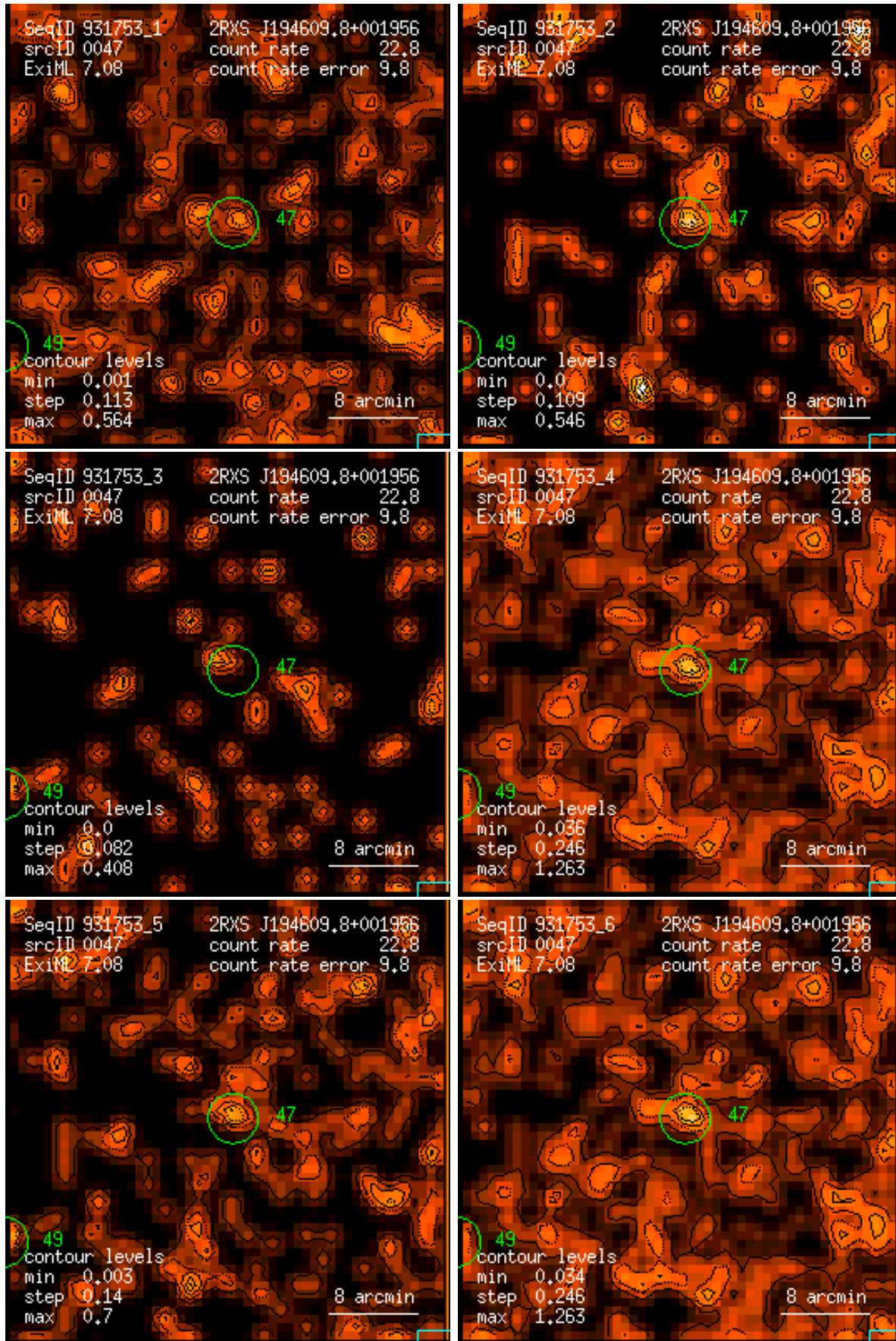
Figure 47: RASS 931753: detection 0047: band rate images, Gaussian filter: (1) PSPC channels 11 – 41, (2) 52 – 90, (3) 91 – 201, (4) 11 – 235, (5) 52 – 201, (6) 11 – 201. Broad band rates in counts/ks. Band rate contour levels in counts/ks/arcmin 2 .
