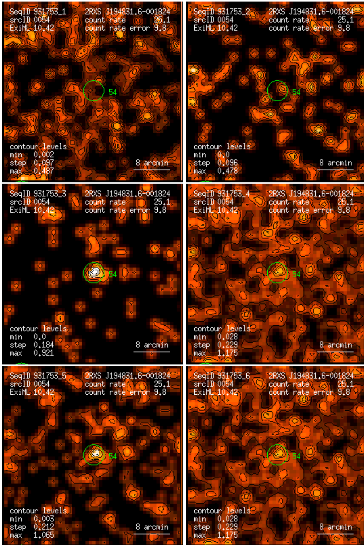
Figure 54: RASS 931753: detection 0054: band rate images, Gaussian filter: (1) PSPC channels 11 – 41, (2) 52 – 90, (3) 91 – 201, (4) 11 – 235, (5) 52 – 201, (6) 11 – 201. Broad band rates in counts/ks. Band rate contour levels in counts/ks/arcmin 2 .
