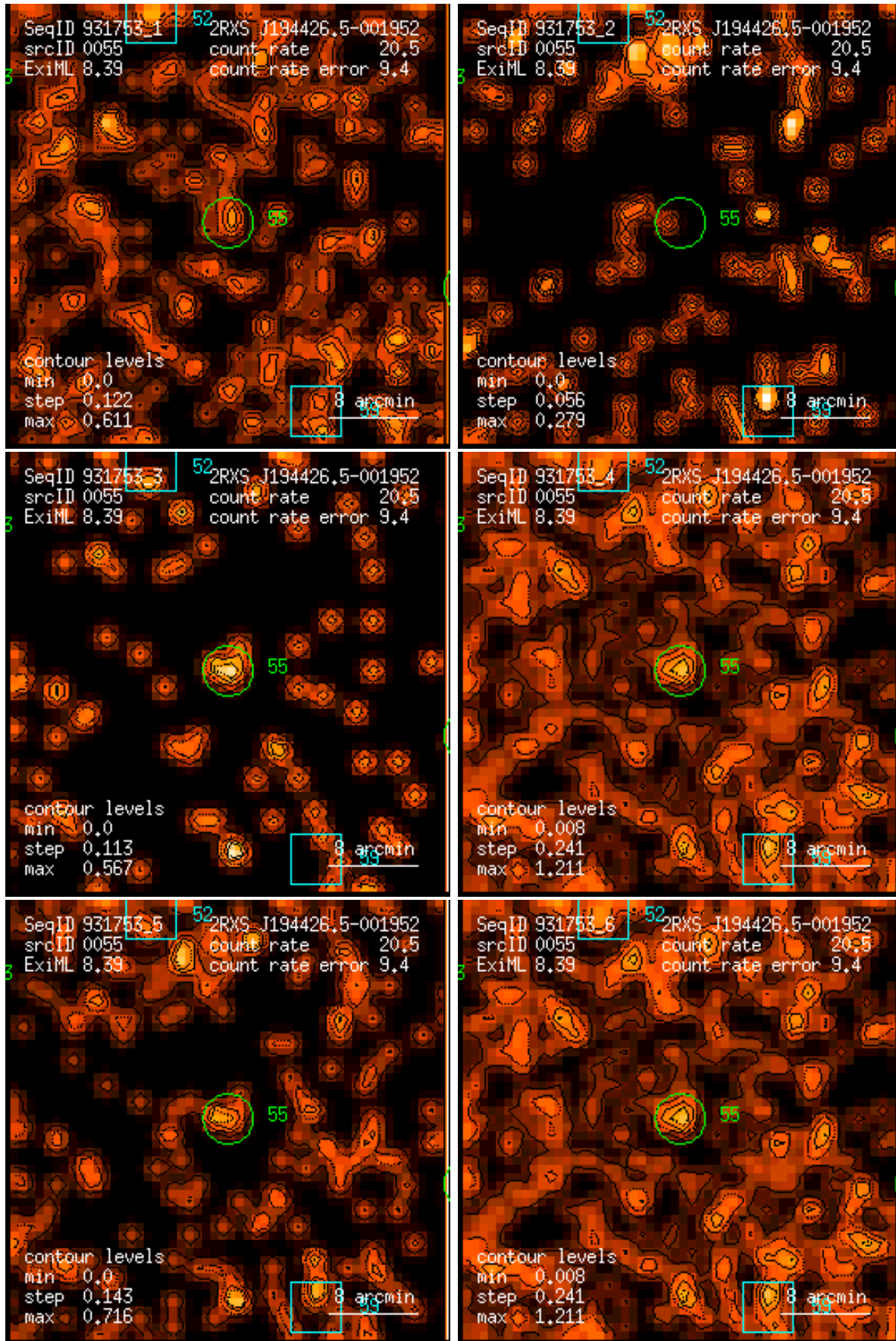
Figure 55: RASS 931753: detection 0055: band rate images, Gaussian filter: (1) PSPC channels 11 – 41, (2) 52 – 90, (3) 91 – 201, (4) 11 – 235, (5) 52 – 201, (6) 11 – 201. Broad band rates in counts/ks. Band rate contour levels in counts/ks/arcmin 2 .
