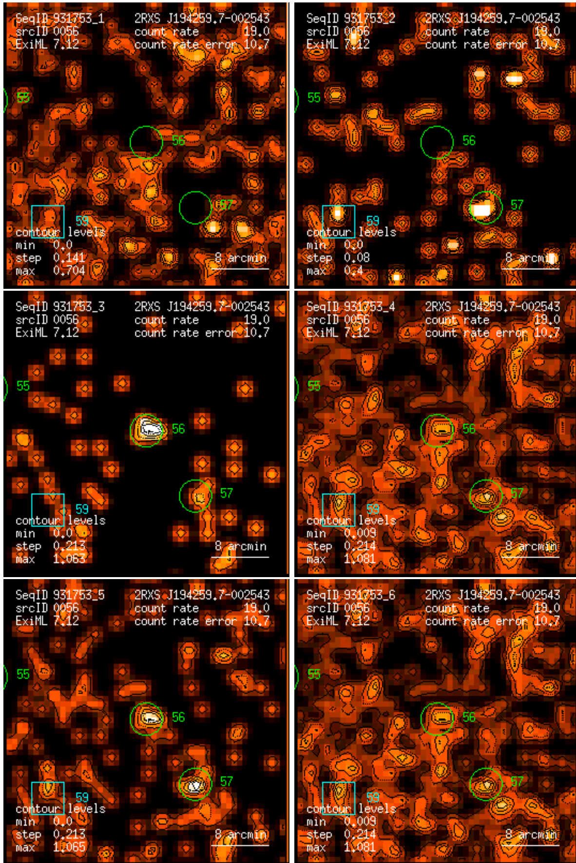
Figure 56: RASS 931753: detection 0056: band rate images, Gaussian filter: (1) PSPC channels 11 – 41, (2) 52 – 90, (3) 91 – 201, (4) 11 – 235, (5) 52 – 201, (6) 11 – 201. Broad band rates in counts/ks. Band rate contour levels in counts/ks/arcmin 2 .
