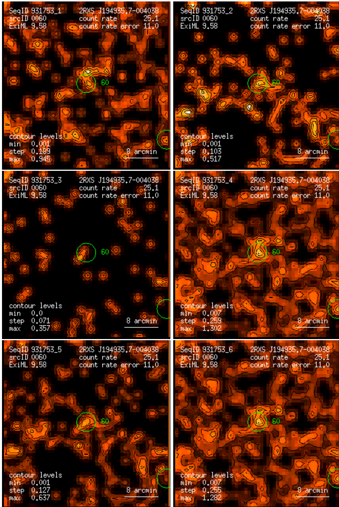
Figure 60: RASS 931753: detection 0060: band rate images, Gaussian filter: (1) PSPC channels 11 – 41, (2) 52 – 90, (3) 91 – 201, (4) 11 – 235, (5) 52 – 201, (6) 11 – 201. Broad band rates in counts/ks. Band rate contour levels in counts/ks/arcmin 2 .
