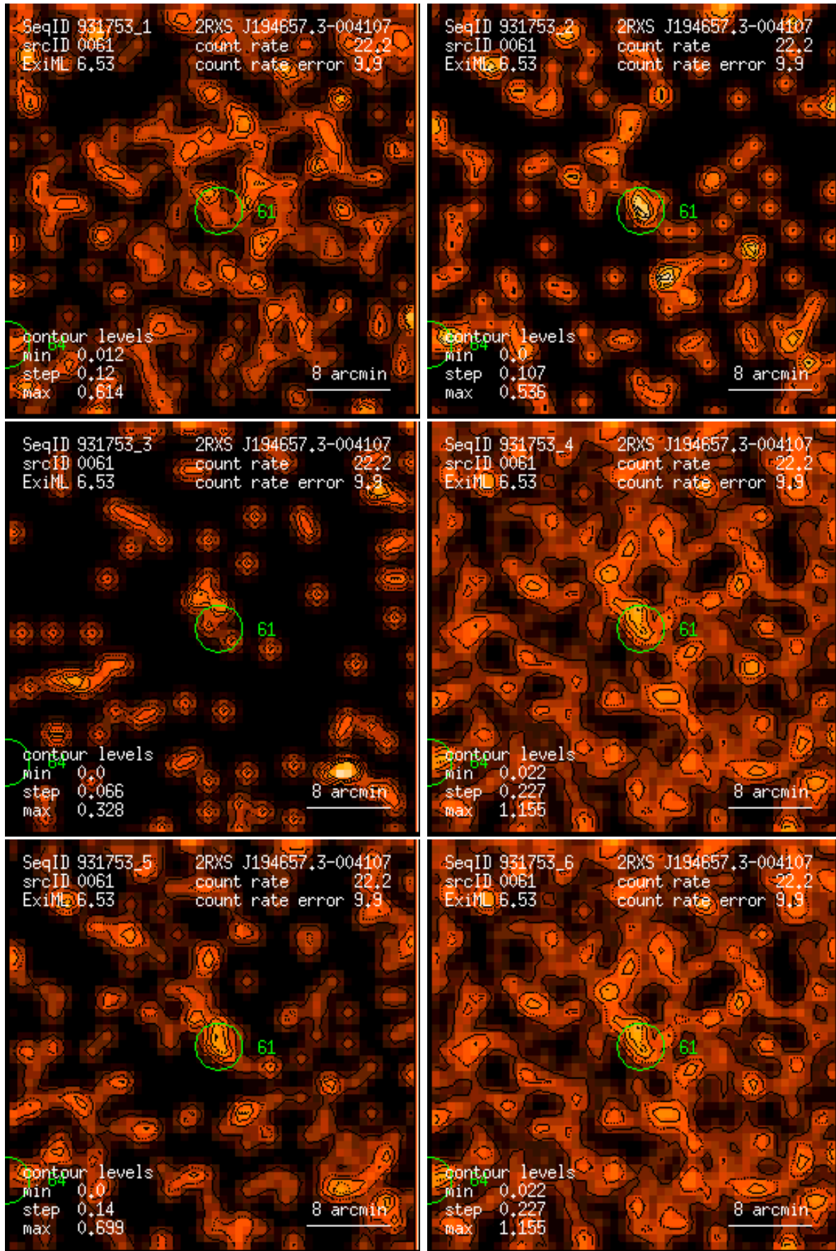
Figure 61: RASS 931753: detection 0061: band rate images, Gaussian filter: (1) PSPC channels 11 – 41, (2) 52 – 90, (3) 91 – 201, (4) 11 – 235, (5) 52 – 201, (6) 11 – 201. Broad band rates in counts/ks. Band rate contour levels in counts/ks/arcmin 2 .
