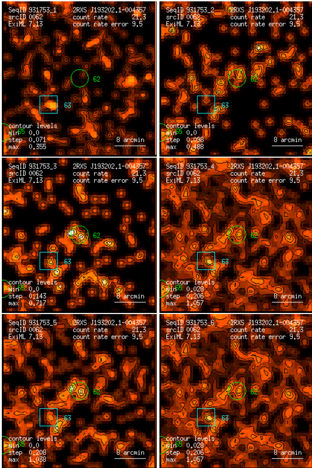
Figure 62: RASS 931753: detection 0062: band rate images, Gaussian filter: (1) PSPC channels 11 – 41, (2) 52 – 90, (3) 91 – 201, (4) 11 – 235, (5) 52 – 201, (6) 11 – 201. Broad band rates in counts/ks. Band rate contour levels in counts/ks/arcmin 2 .
