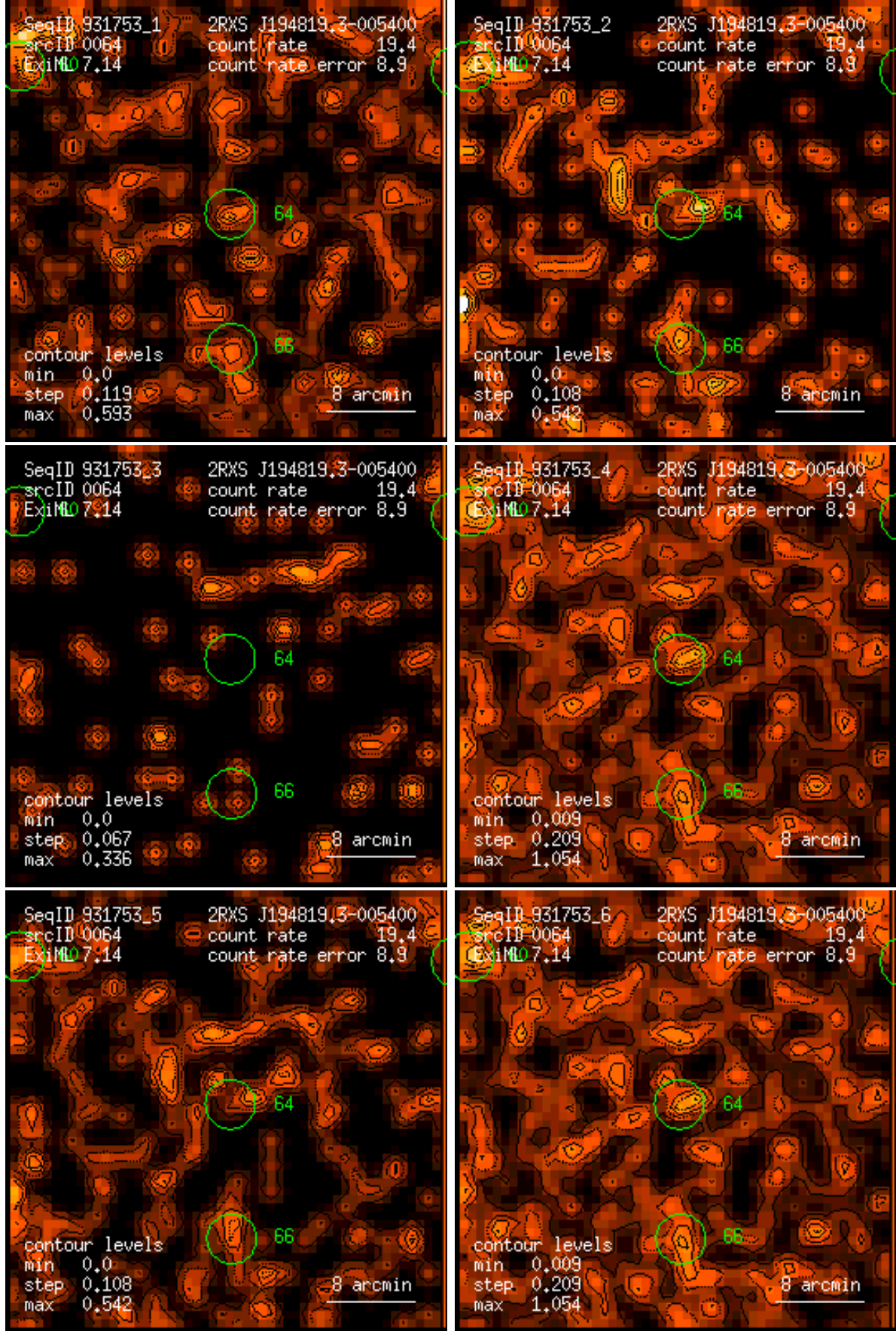
Figure 64: RASS 931753: detection 0064: band rate images, Gaussian filter: (1) PSPC channels 11 – 41, (2) 52 – 90, (3) 91 – 201, (4) 11 – 235, (5) 52 – 201, (6) 11 – 201. Broad band rates in counts/ks. Band rate contour levels in counts/ks/arcmin 2 .
