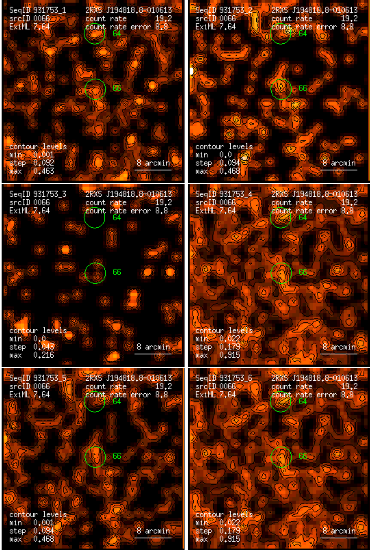
Figure 66: RASS 931753: detection 0066: band rate images, Gaussian filter: (1) PSPC channels 11 – 41, (2) 52 – 90, (3) 91 – 201, (4) 11 – 235, (5) 52 – 201, (6) 11 – 201. Broad band rates in counts/ks. Band rate contour levels in counts/ks/arcmin 2 .
