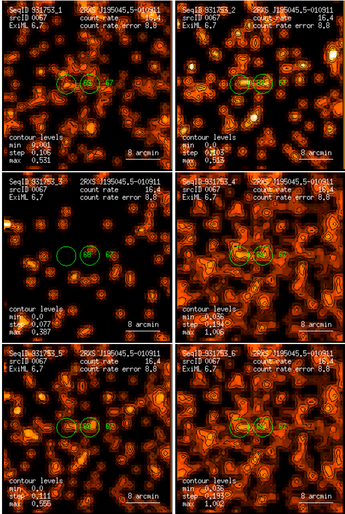
Figure 67: RASS 931753: detection 0067: band rate images, Gaussian filter: (1) PSPC channels 11 – 41, (2) 52 – 90, (3) 91 – 201, (4) 11 – 235, (5) 52 – 201, (6) 11 – 201. Broad band rates in counts/ks. Band rate contour levels in counts/ks/arcmin 2 .
