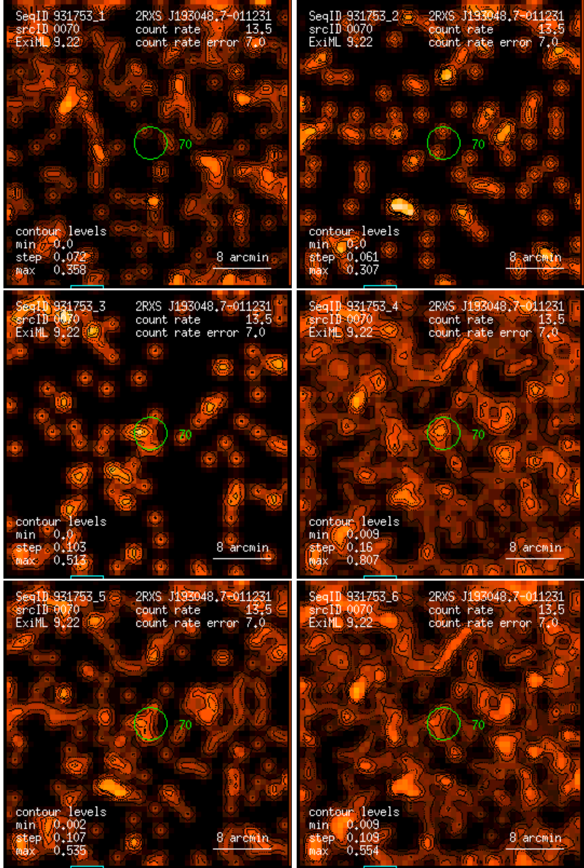
Figure 70: RASS 931753: detection 0070: band rate images, Gaussian filter: (1) PSPC channels 11 – 41, (2) 52 – 90, (3) 91 – 201, (4) 11 – 235, (5) 52 – 201, (6) 11 – 201. Broad band rates in counts/ks. Band rate contour levels in counts/ks/arcmin 2 .
