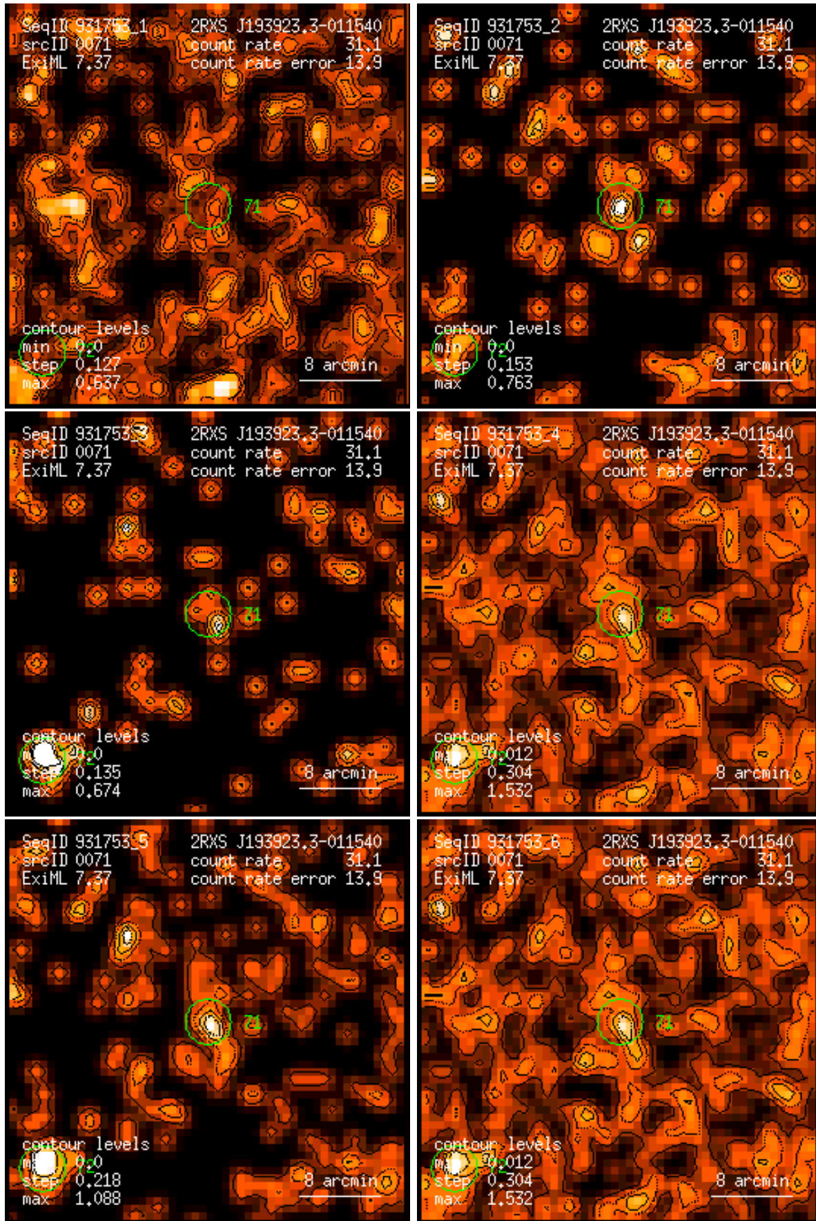
Figure 71: RASS 931753: detection 0071: band rate images, Gaussian filter: (1) PSPC channels 11 – 41, (2) 52 – 90, (3) 91 – 201, (4) 11 – 235, (5) 52 – 201, (6) 11 – 201. Broad band rates in counts/ks. Band rate contour levels in counts/ks/arcmin 2 .
