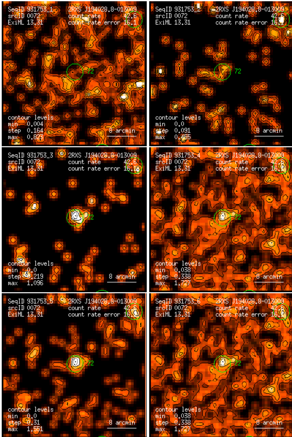
Figure 72: RASS 931753: detection 0072: band rate images, Gaussian filter: (1) PSPC channels 11 – 41, (2) 52 – 90, (3) 91 – 201, (4) 11 – 235, (5) 52 – 201, (6) 11 – 201. Broad band rates in counts/ks. Band rate contour levels in counts/ks/arcmin 2 .
