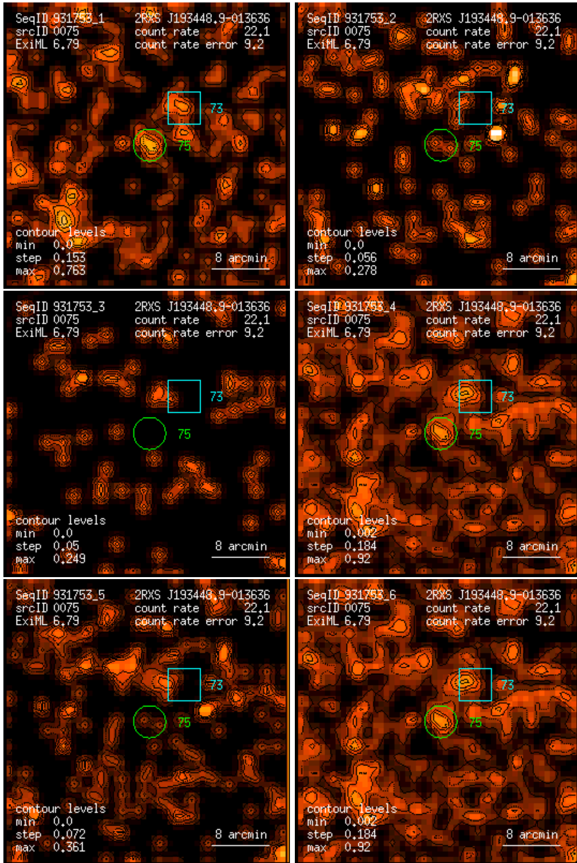
Figure 75: RASS 931753: detection 0075: band rate images, Gaussian filter: (1) PSPC channels 11 – 41, (2) 52 – 90, (3) 91 – 201, (4) 11 – 235, (5) 52 – 201, (6) 11 – 201. Broad band rates in counts/ks. Band rate contour levels in counts/ks/arcmin 2 .
