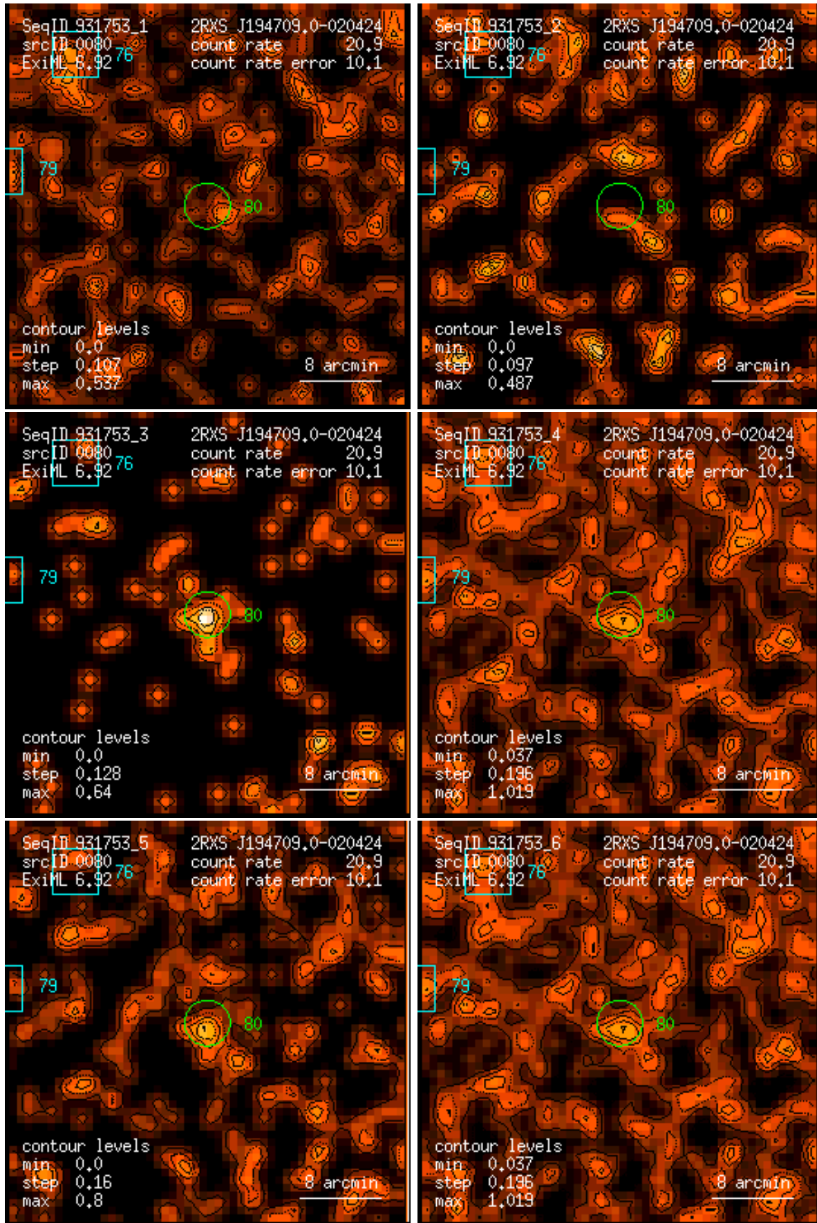
Figure 80: RASS 931753: detection 0080: band rate images, Gaussian filter: (1) PSPC channels 11 – 41, (2) 52 – 90, (3) 91 – 201, (4) 11 – 235, (5) 52 – 201, (6) 11 – 201. Broad band rates in counts/ks. Band rate contour levels in counts/ks/arcmin 2 .
