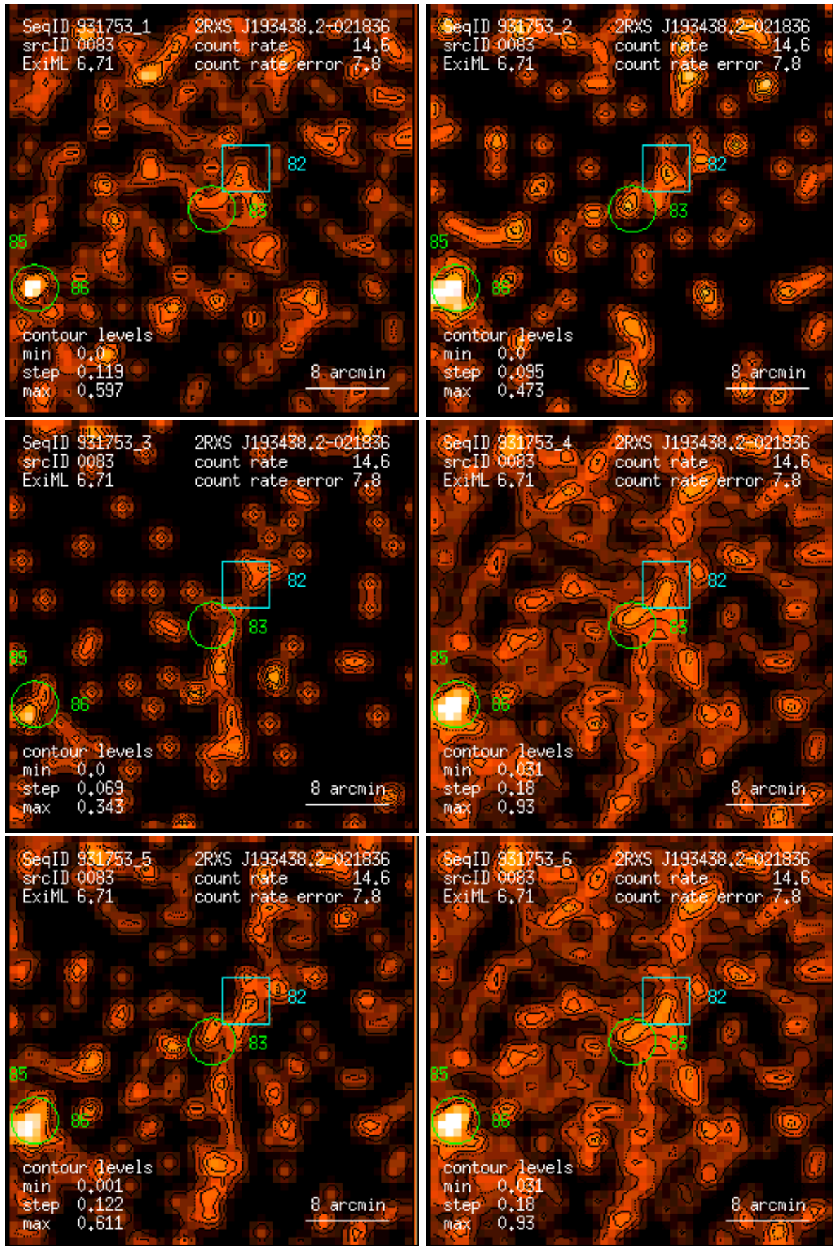
Figure 83: RASS 931753: detection 0083: band rate images, Gaussian filter: (1) PSPC channels 11 – 41, (2) 52 – 90, (3) 91 – 201, (4) 11 – 235, (5) 52 – 201, (6) 11 – 201. Broad band rates in counts/ks. Band rate contour levels in counts/ks/arcmin 2 .
