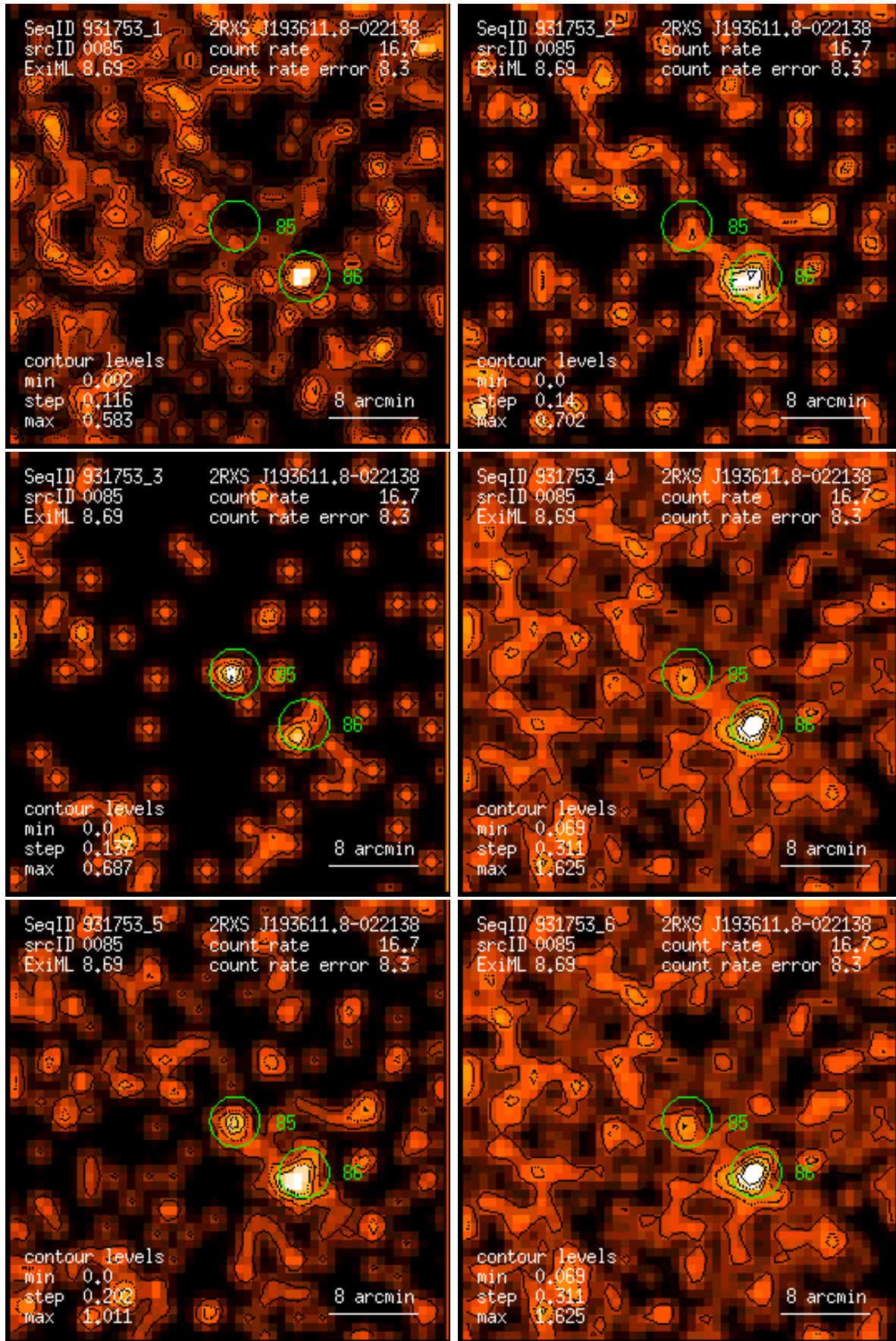
Figure 85: RASS 931753: detection 0085: band rate images, Gaussian filter: (1) PSPC channels 11 – 41, (2) 52 – 90, (3) 91 – 201, (4) 11 – 235, (5) 52 – 201, (6) 11 – 201. Broad band rates in counts/ks. Band rate contour levels in counts/ks/arcmin 2 .
