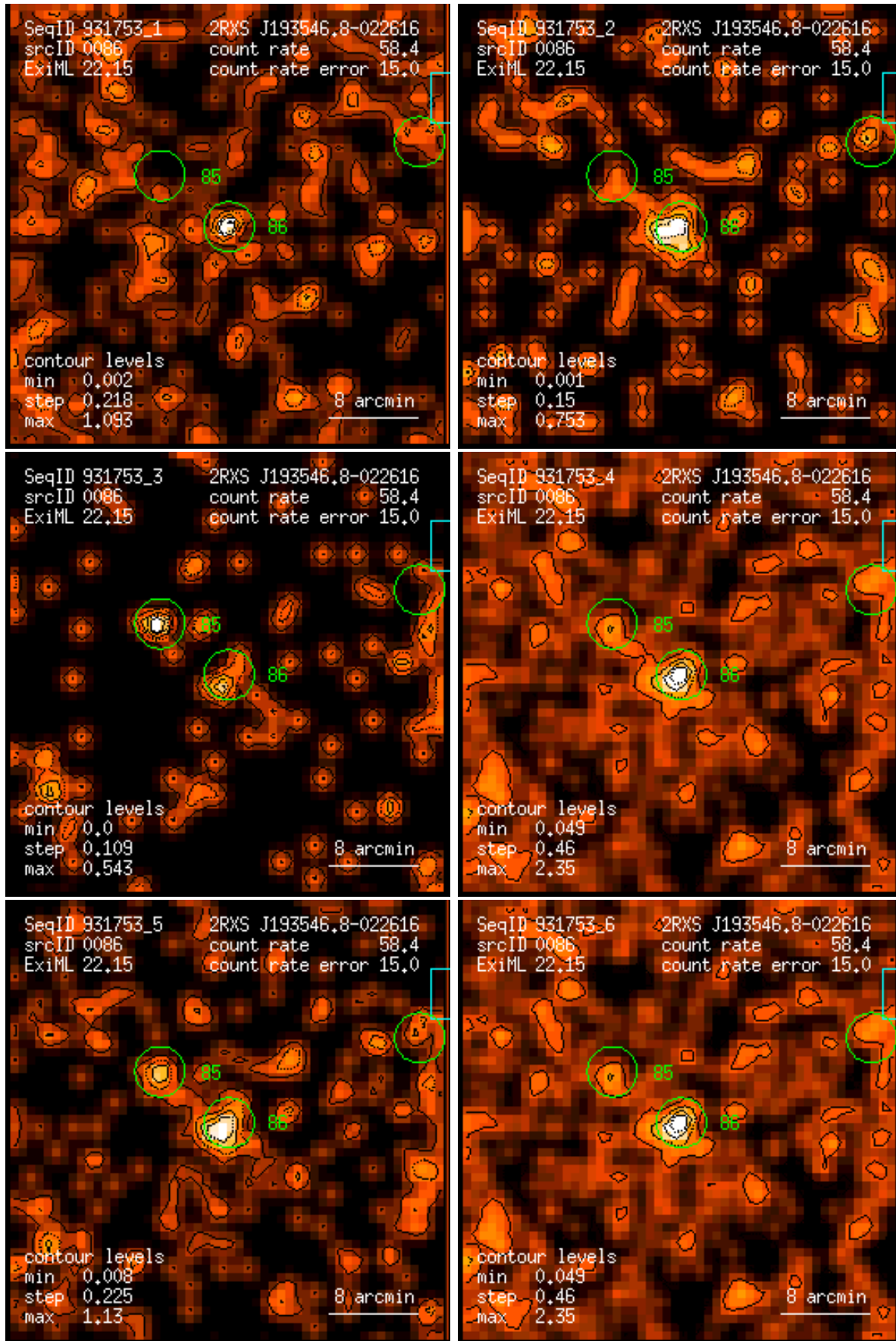
Figure 86: RASS 931753: detection 0086: band rate images, Gaussian filter: (1) PSPC channels 11 – 41, (2) 52 – 90, (3) 91 – 201, (4) 11 – 235, (5) 52 – 201, (6) 11 – 201. Broad band rates in counts/ks. Band rate contour levels in counts/ks/arcmin 2 .
