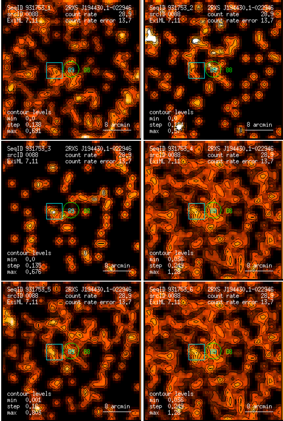
Figure 88: RASS 931753: detection 0088: band rate images, Gaussian filter: (1) PSPC channels 11 – 41, (2) 52 – 90, (3) 91 – 201, (4) 11 – 235, (5) 52 – 201, (6) 11 – 201. Broad band rates in counts/ks. Band rate contour levels in counts/ks/arcmin 2 .
