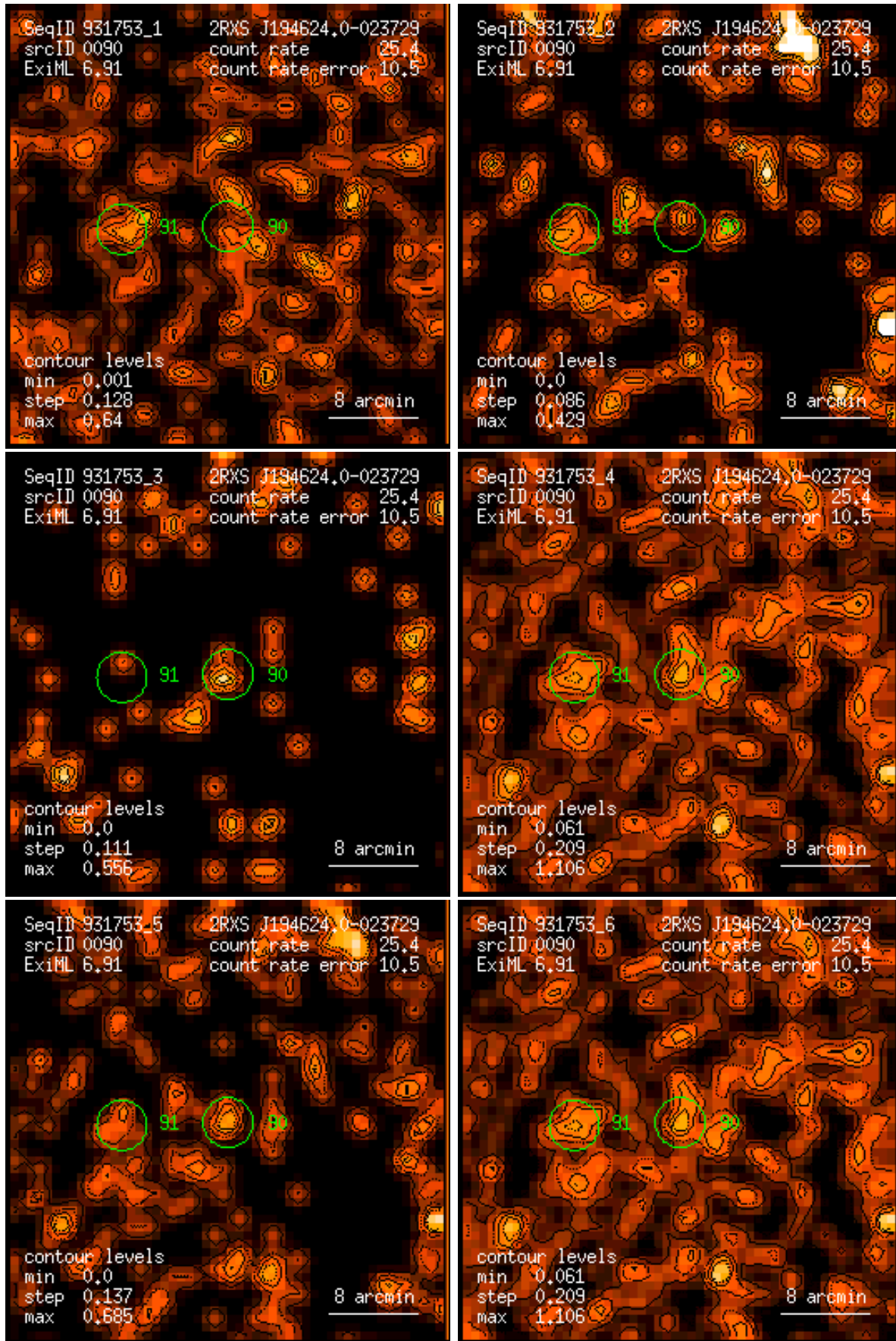
Figure 90: RASS 931753: detection 0090: band rate images, Gaussian filter: (1) PSPC channels 11 – 41, (2) 52 – 90, (3) 91 – 201, (4) 11 – 235, (5) 52 – 201, (6) 11 – 201. Broad band rates in counts/ks. Band rate contour levels in counts/ks/arcmin 2 .
