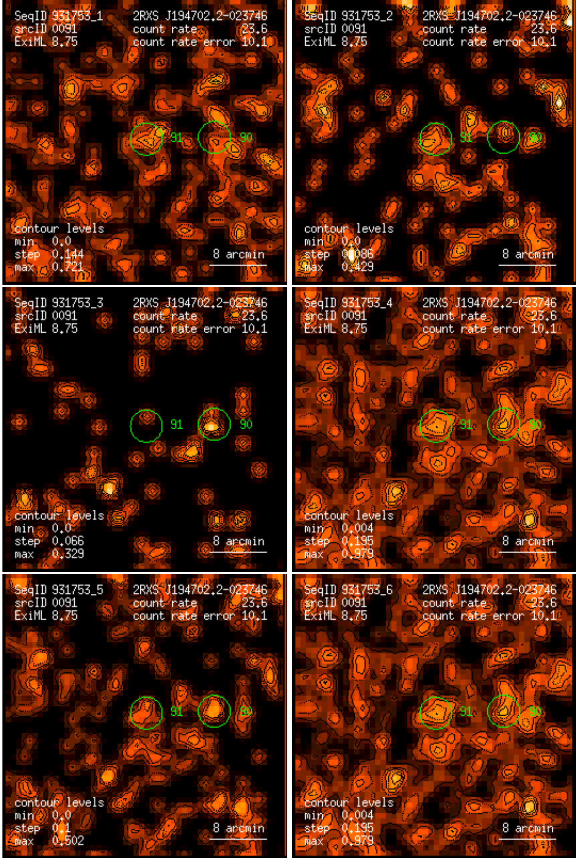
Figure 91: RASS 931753: detection 0091: band rate images, Gaussian filter: (1) PSPC channels 11 – 41, (2) 52 – 90, (3) 91 – 201, (4) 11 – 235, (5) 52 – 201, (6) 11 – 201. Broad band rates in counts/ks. Band rate contour levels in counts/ks/arcmin 2 .
