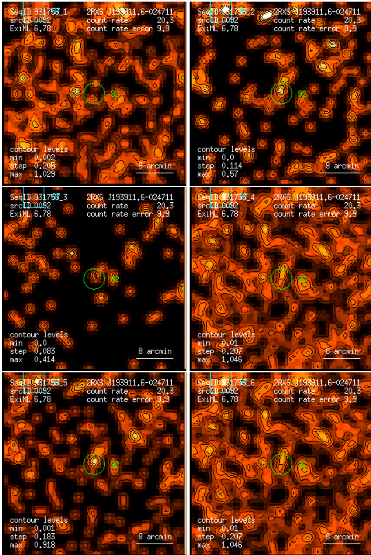
Figure 92: RASS 931753: detection 0092: band rate images, Gaussian filter: (1) PSPC channels 11 – 41, (2) 52 – 90, (3) 91 – 201, (4) 11 – 235, (5) 52 – 201, (6) 11 – 201. Broad band rates in counts/ks. Band rate contour levels in counts/ks/arcmin 2 .
