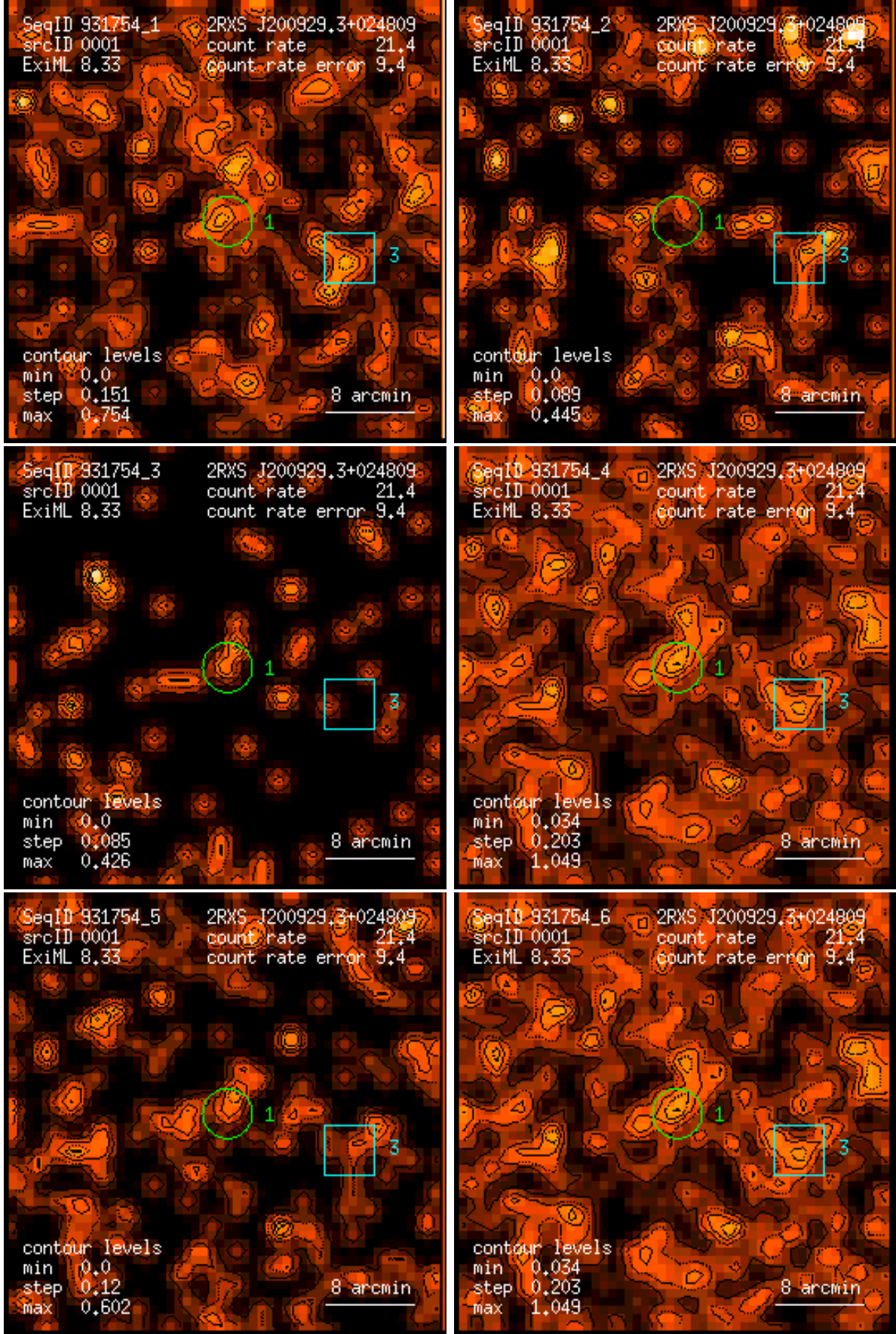
Figure 1: RASS 931754: detection 0001: band rate images, Gaussian filter: (1) PSPC channels 11 – 41, (2) 52 – 90, (3) 91 – 201, (4) 11 – 235, (5) 52 – 201, (6) 11 – 201. Broad band rates in counts/ks. Band rate contour levels in counts/ks/arcmin 2 .
