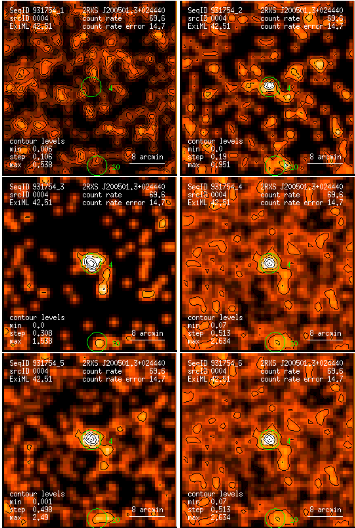
Figure 4: RASS 931754: detection 0004: band rate images, Gaussian filter: (1) PSPC channels 11 – 41, (2) 52 – 90, (3) 91 – 201, (4) 11 – 235, (5) 52 – 201, (6) 11 – 201. Broad band rates in counts/ks. Band rate contour levels in counts/ks/arcmin 2 .
