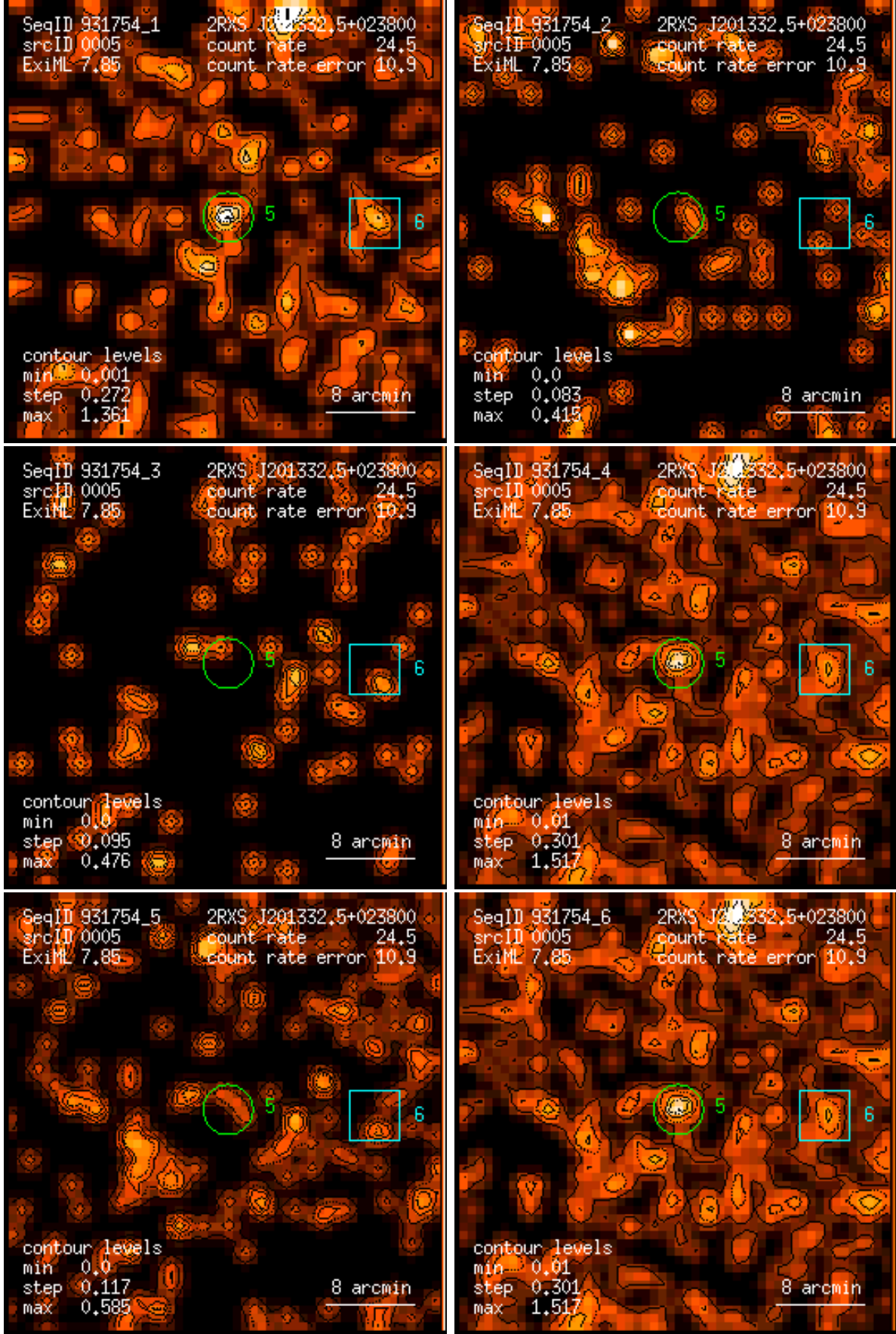
Figure 5: RASS 931754: detection 0005: band rate images, Gaussian filter: (1) PSPC channels 11 – 41, (2) 52 – 90, (3) 91 – 201, (4) 11 – 235, (5) 52 – 201, (6) 11 – 201. Broad band rates in counts/ks. Band rate contour levels in counts/ks/arcmin 2 .
