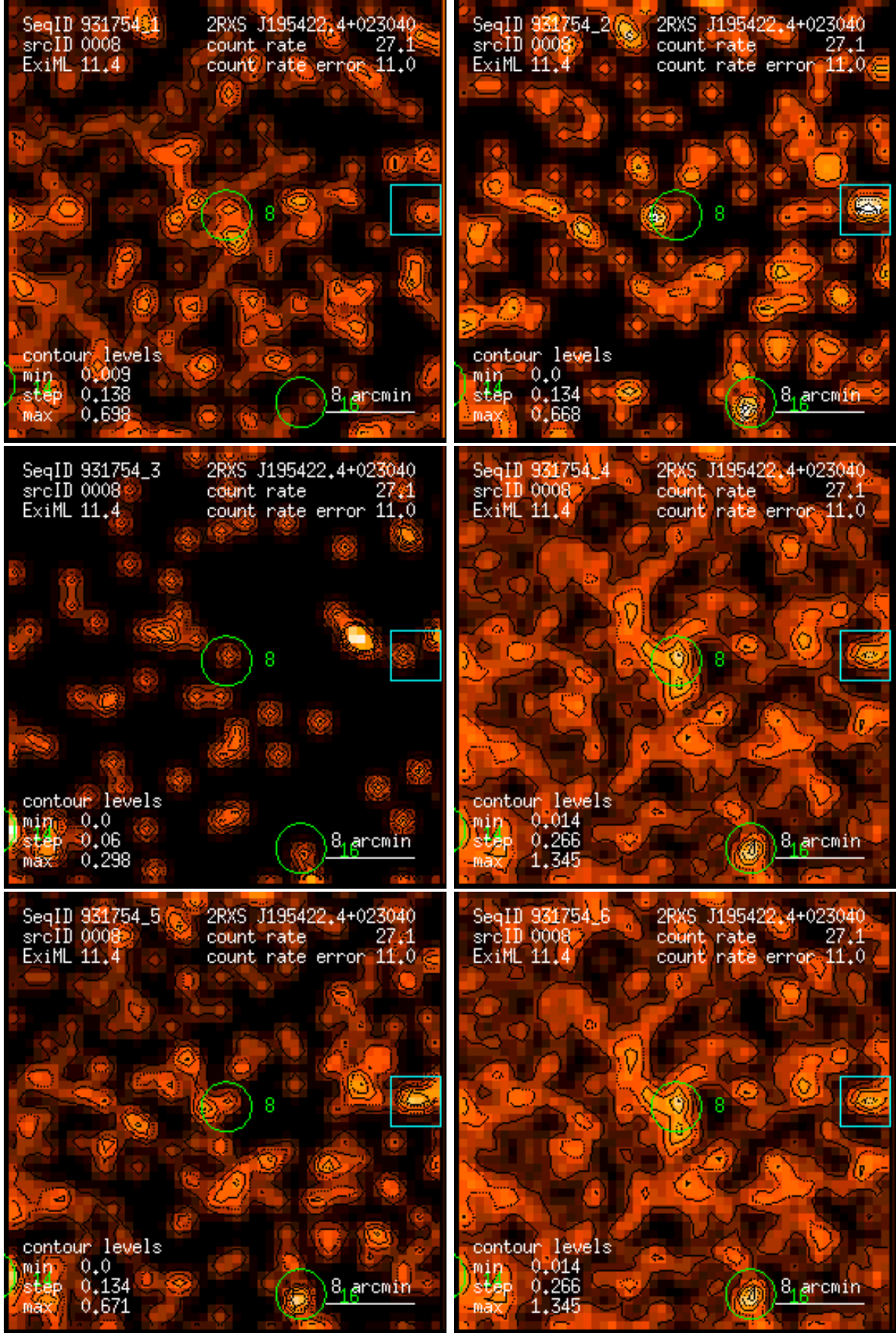
Figure 8: RASS 931754: detection 0008: band rate images, Gaussian filter: (1) PSPC channels 11 – 41, (2) 52 – 90, (3) 91 – 201, (4) 11 – 235, (5) 52 – 201, (6) 11 – 201. Broad band rates in counts/ks. Band rate contour levels in counts/ks/arcmin 2 .
