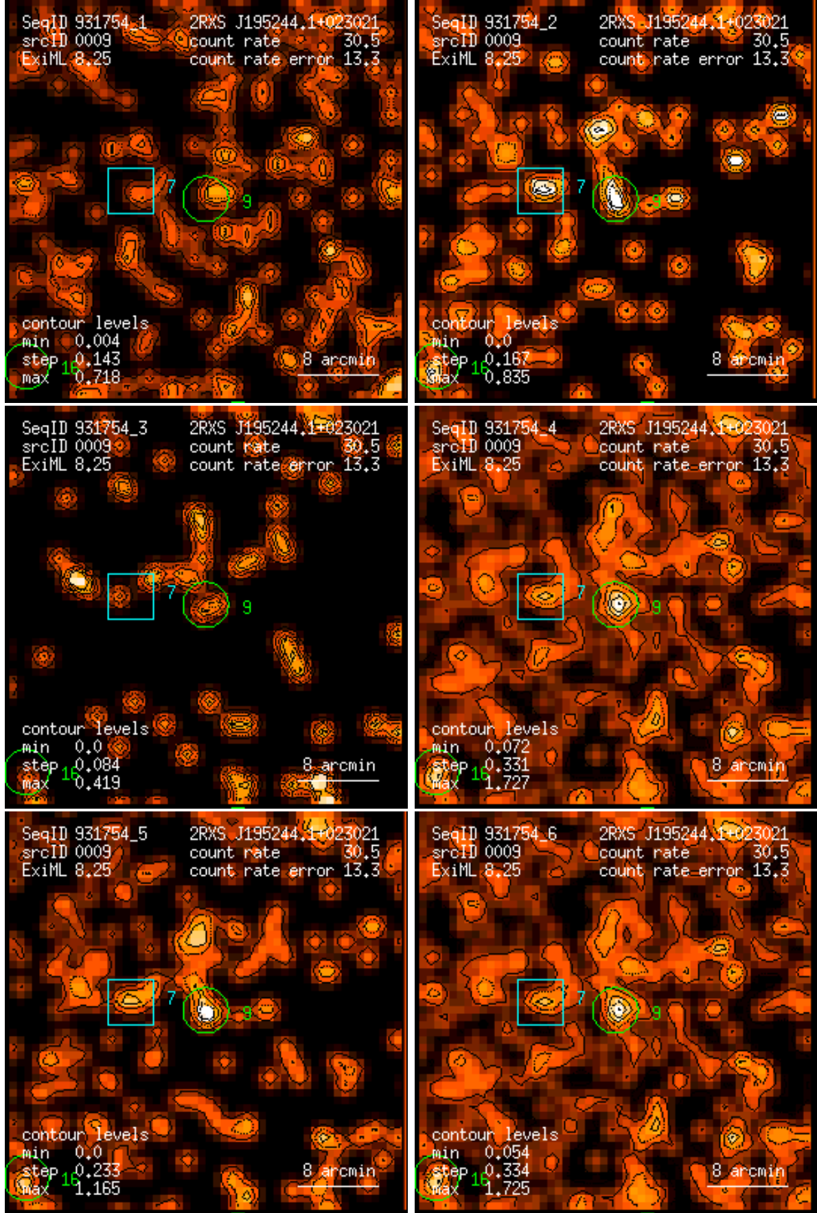
Figure 9: RASS 931754: detection 0009: band rate images, Gaussian filter: (1) PSPC channels 11 – 41, (2) 52 – 90, (3) 91 – 201, (4) 11 – 235, (5) 52 – 201, (6) 11 – 201. Broad band rates in counts/ks. Band rate contour levels in counts/ks/arcmin 2 .
