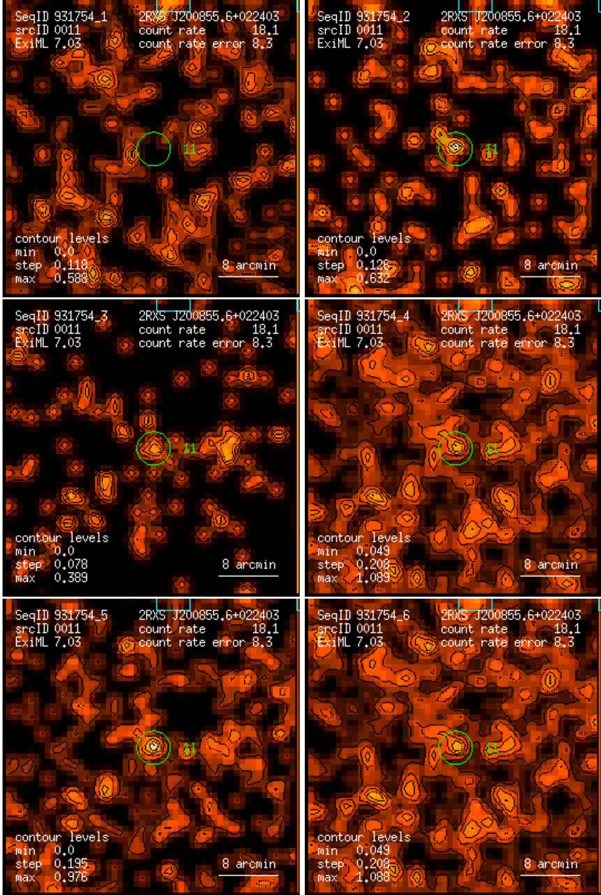
Figure 11: RASS 931754: detection 0011: band rate images, Gaussian filter: (1) PSPC channels 11 – 41, (2) 52 – 90, (3) 91 – 201, (4) 11 – 235, (5) 52 – 201, (6) 11 – 201. Broad band rates in counts/ks. Band rate contour levels in counts/ks/arcmin 2 .
