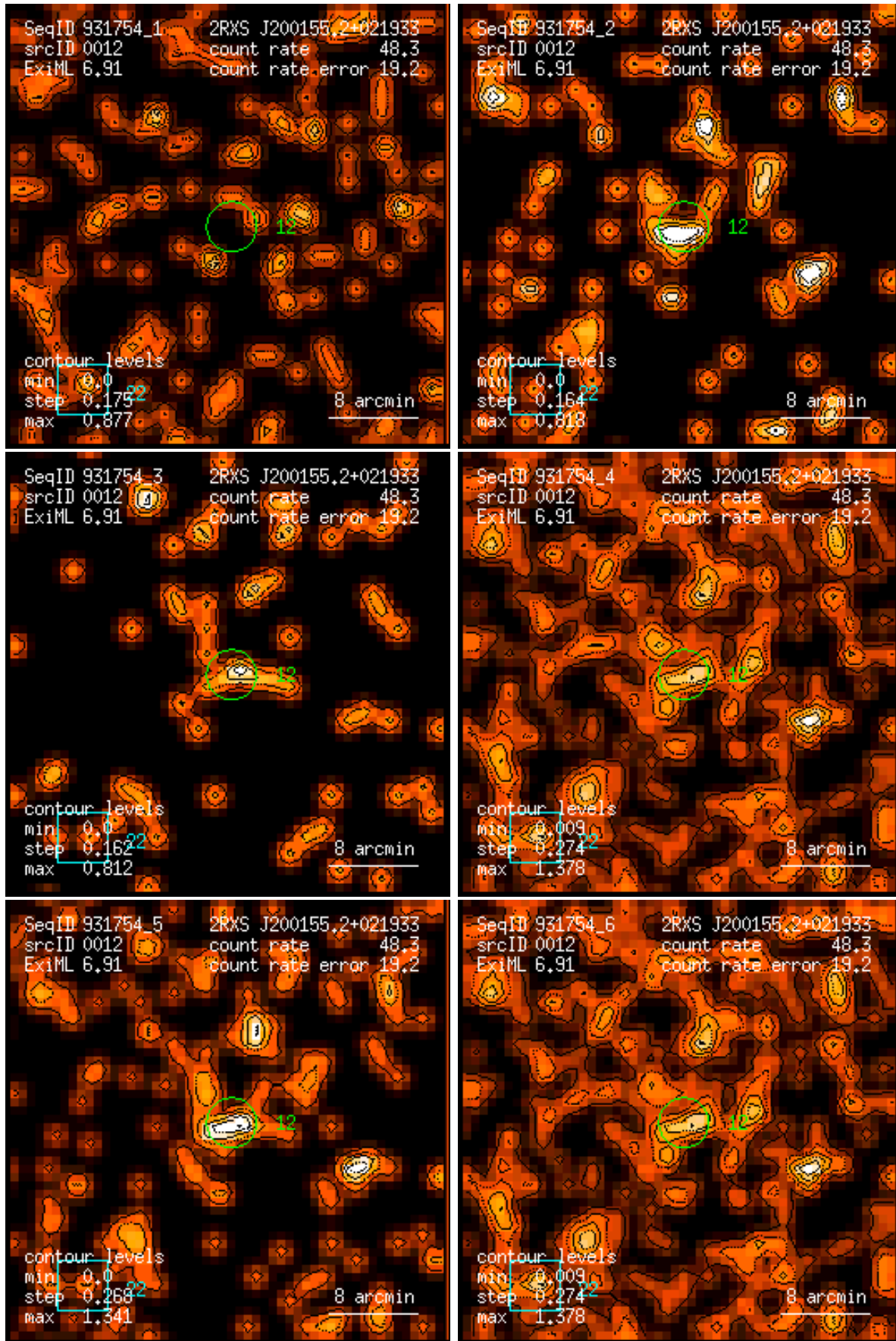
Figure 12: RASS 931754: detection 0012: band rate images, Gaussian filter: (1) PSPC channels 11 – 41, (2) 52 – 90, (3) 91 – 201, (4) 11 – 235, (5) 52 – 201, (6) 11 – 201. Broad band rates in counts/ks. Band rate contour levels in counts/ks/arcmin 2 .
