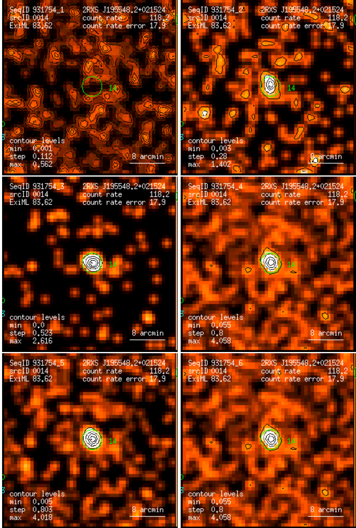
Figure 14: RASS 931754: detection 0014: band rate images, Gaussian filter: (1) PSPC channels 11 – 41, (2) 52 – 90, (3) 91 – 201, (4) 11 – 235, (5) 52 – 201, (6) 11 – 201. Broad band rates in counts/ks. Band rate contour levels in counts/ks/arcmin 2 .
