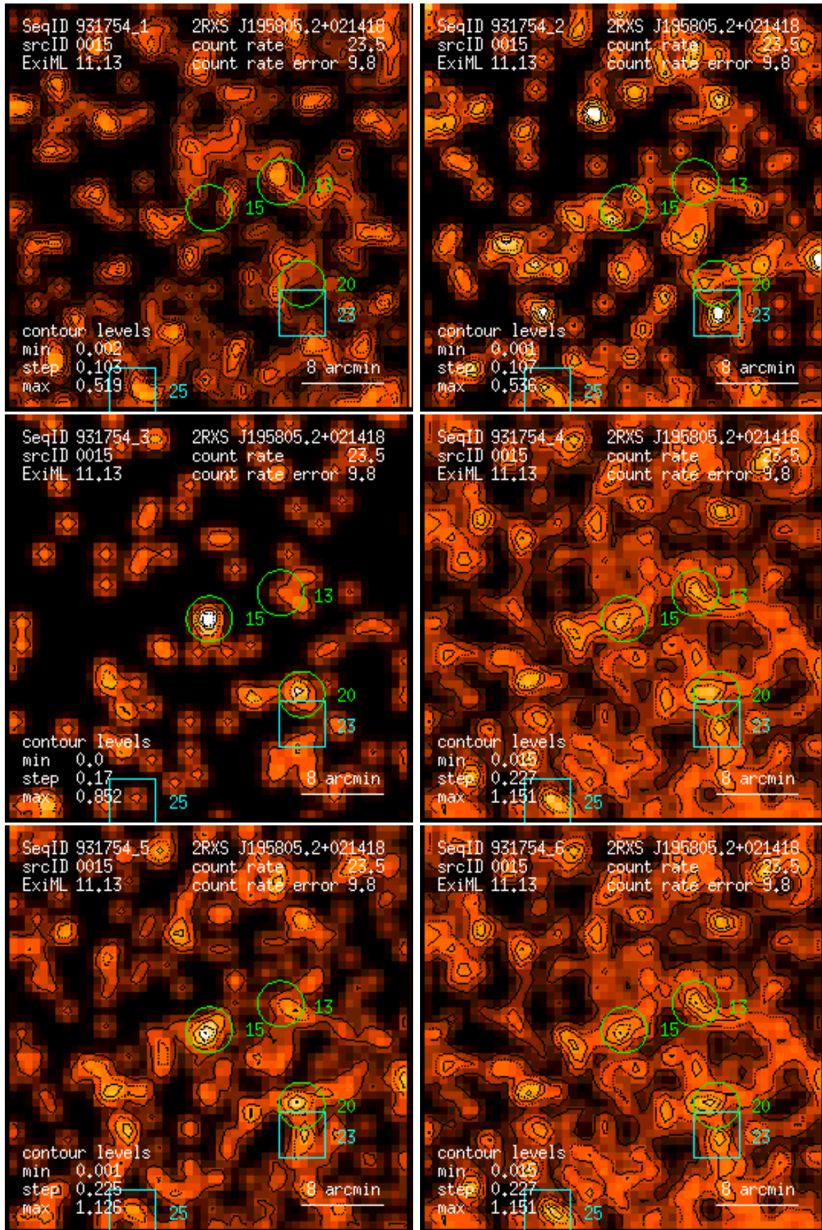
Figure 15: RASS 931754: detection 0015: band rate images, Gaussian filter: (1) PSPC channels 11 – 41, (2) 52 – 90, (3) 91 – 201, (4) 11 – 235, (5) 52 – 201, (6) 11 – 201. Broad band rates in counts/ks. Band rate contour levels in counts/ks/arcmin 2 .
