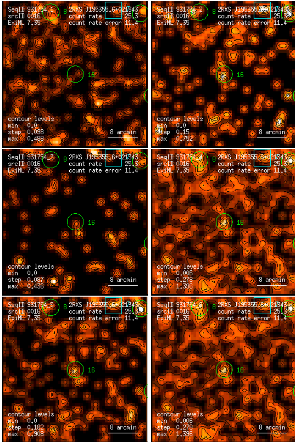
Figure 16: RASS 931754: detection 0016: band rate images, Gaussian filter: (1) PSPC channels 11 – 41, (2) 52 – 90, (3) 91 – 201, (4) 11 – 235, (5) 52 – 201, (6) 11 – 201. Broad band rates in counts/ks. Band rate contour levels in counts/ks/arcmin 2 .
