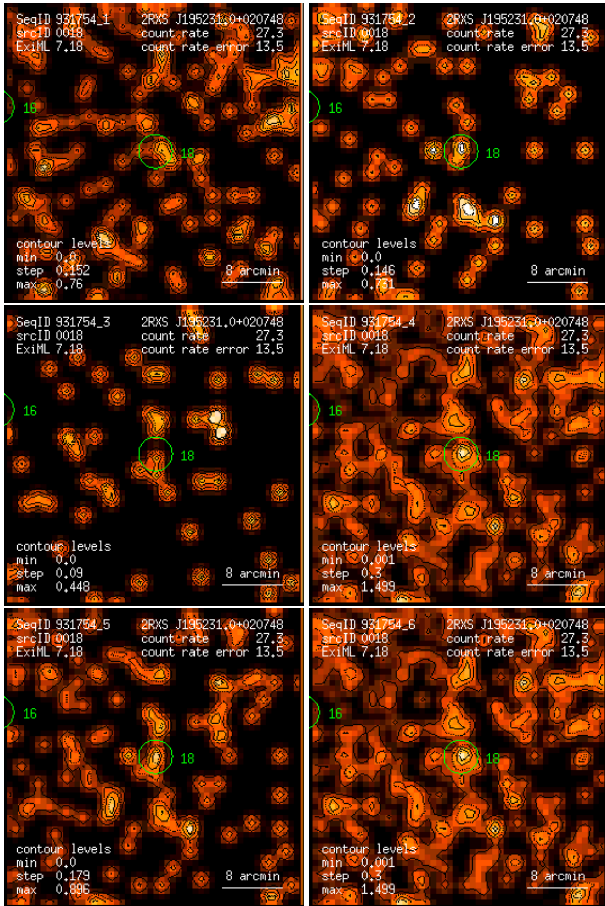
Figure 18: RASS 931754: detection 0018: band rate images, Gaussian filter: (1) PSPC channels 11 – 41, (2) 52 – 90, (3) 91 – 201, (4) 11 – 235, (5) 52 – 201, (6) 11 – 201. Broad band rates in counts/ks. Band rate contour levels in counts/ks/arcmin 2 .
