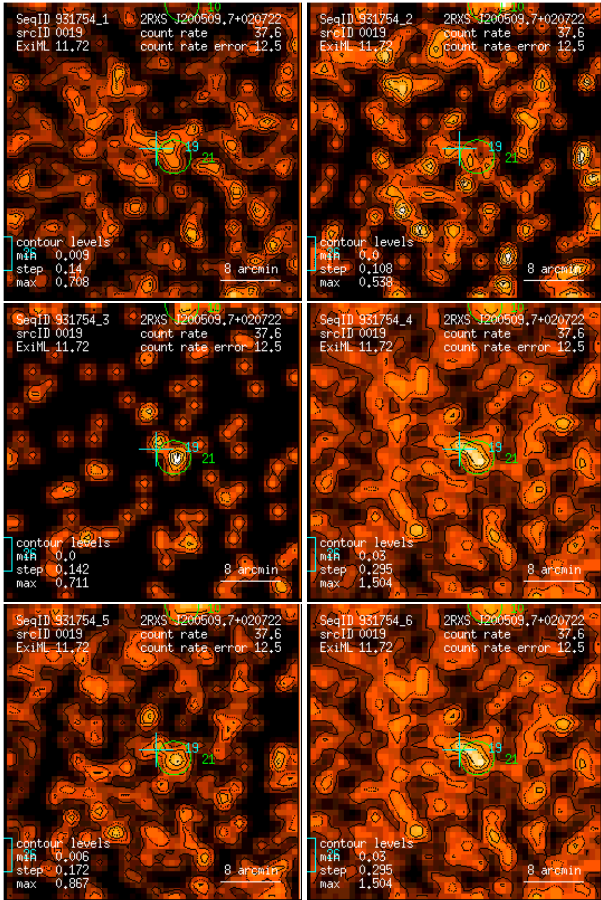
Figure 19: RASS 931754: detection 0019: band rate images, Gaussian filter: (1) PSPC channels 11 – 41, (2) 52 – 90, (3) 91 – 201, (4) 11 – 235, (5) 52 – 201, (6) 11 – 201. Broad band rates in counts/ks. Band rate contour levels in counts/ks/arcmin 2 .
