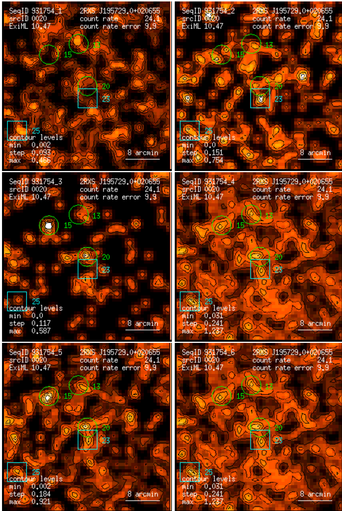
Figure 20: RASS 931754: detection 0020: band rate images, Gaussian filter: (1) PSPC channels 11 – 41, (2) 52 – 90, (3) 91 – 201, (4) 11 – 235, (5) 52 – 201, (6) 11 – 201. Broad band rates in counts/ks. Band rate contour levels in counts/ks/arcmin 2 .
