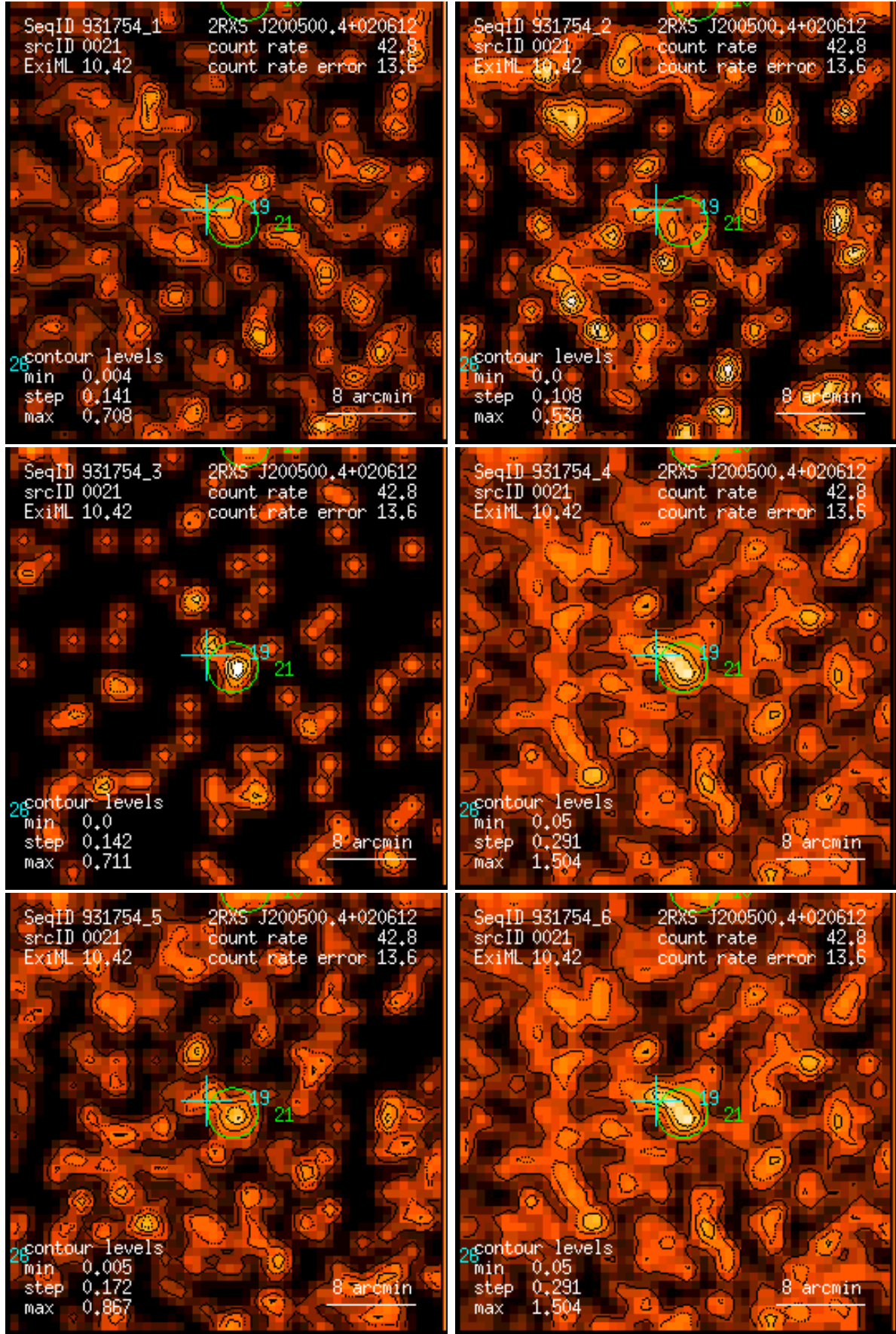
Figure 21: RASS 931754: detection 0021: band rate images, Gaussian filter: (1) PSPC channels 11 – 41, (2) 52 – 90, (3) 91 – 201, (4) 11 – 235, (5) 52 – 201, (6) 11 – 201. Broad band rates in counts/ks. Band rate contour levels in counts/ks/arcmin 2 .
