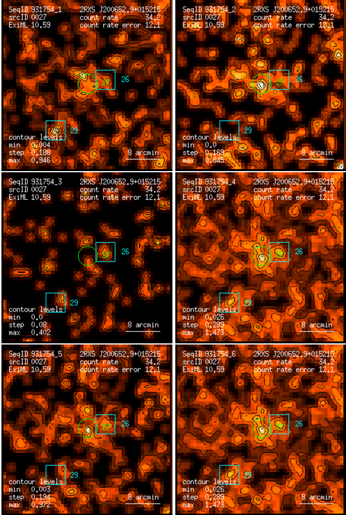
Figure 27: RASS 931754: detection 0027: band rate images, Gaussian filter: (1) PSPC channels 11 – 41, (2) 52 – 90, (3) 91 – 201, (4) 11 – 235, (5) 52 – 201, (6) 11 – 201. Broad band rates in counts/ks. Band rate contour levels in counts/ks/arcmin 2 .
