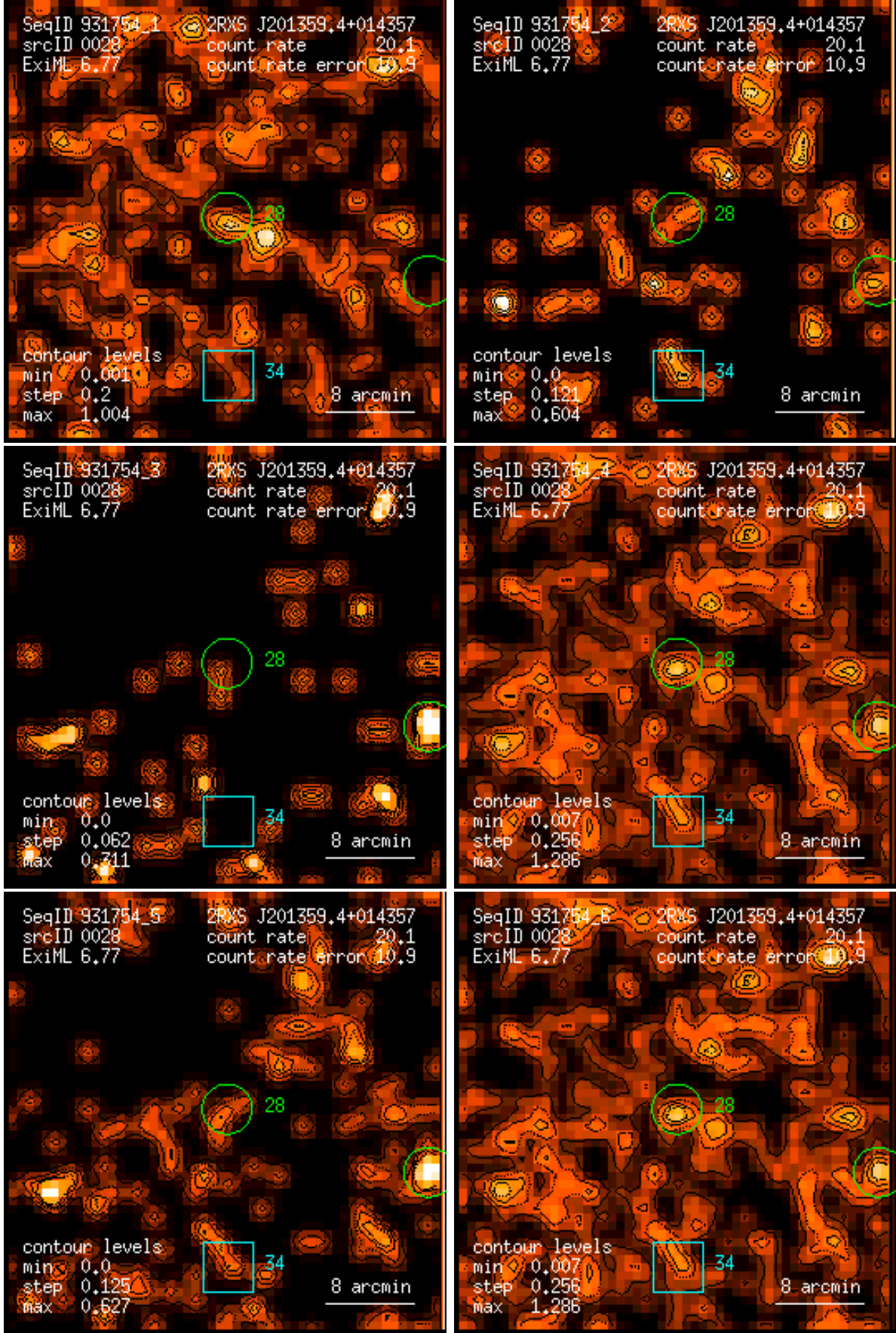
Figure 28: RASS 931754: detection 0028: band rate images, Gaussian filter: (1) PSPC channels 11 – 41, (2) 52 – 90, (3) 91 – 201, (4) 11 – 235, (5) 52 – 201, (6) 11 – 201. Broad band rates in counts/ks. Band rate contour levels in counts/ks/arcmin 2 .
