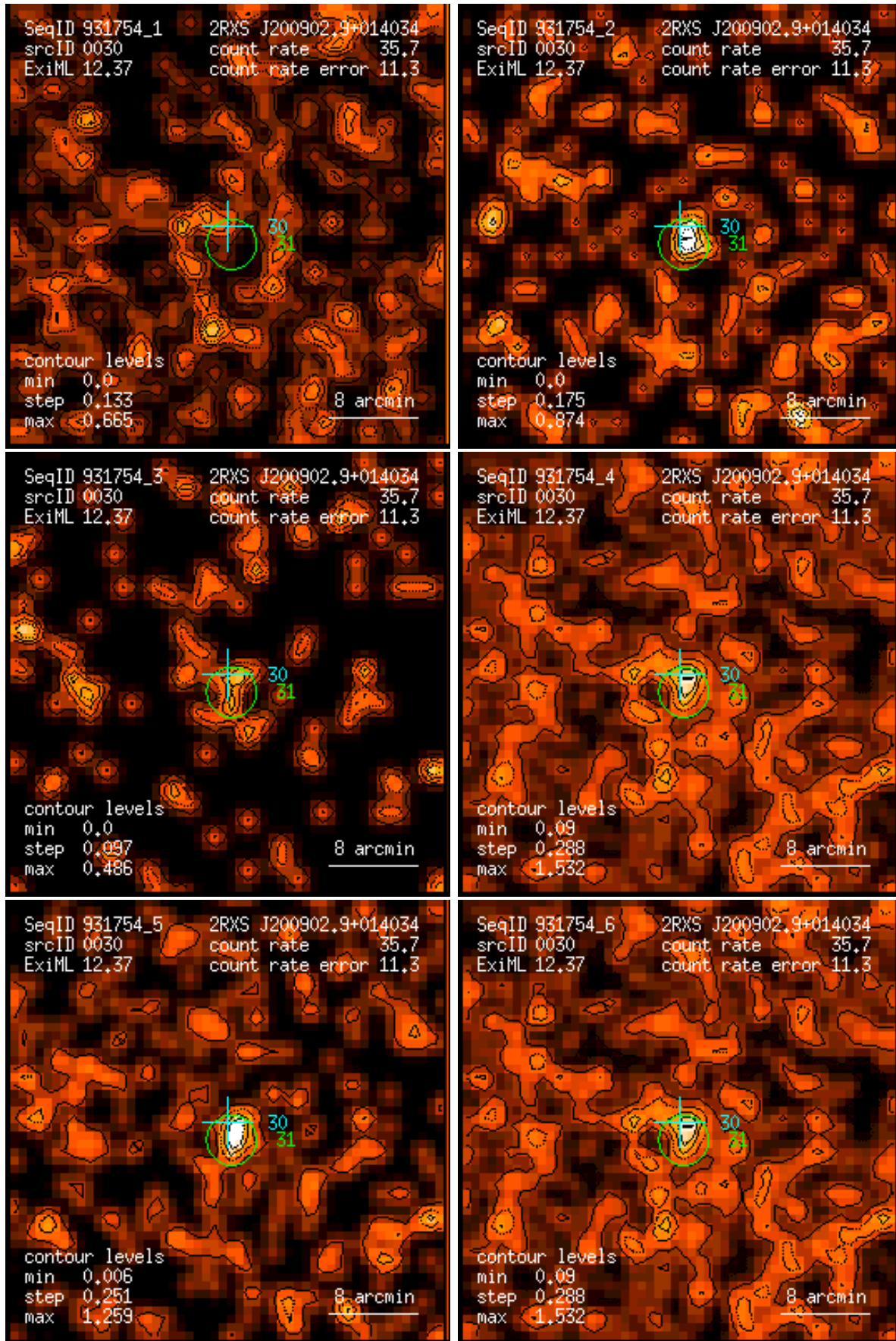
Figure 30: RASS 931754: detection 0030: band rate images, Gaussian filter: (1) PSPC channels 11 – 41, (2) 52 – 90, (3) 91 – 201, (4) 11 – 235, (5) 52 – 201, (6) 11 – 201. Broad band rates in counts/ks. Band rate contour levels in counts/ks/arcmin 2 .
