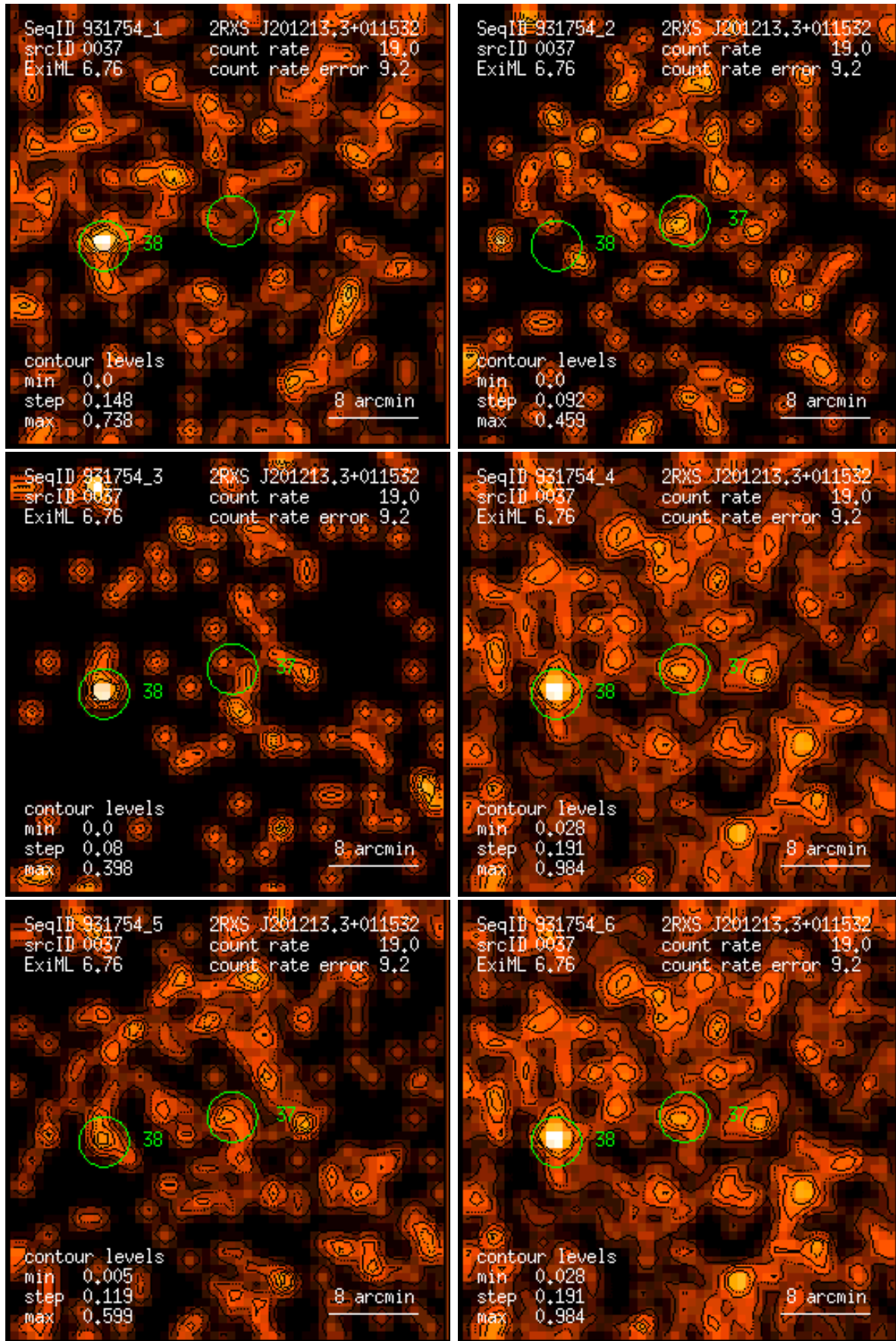
Figure 37: RASS 931754: detection 0037: band rate images, Gaussian filter: (1) PSPC channels 11 – 41, (2) 52 – 90, (3) 91 – 201, (4) 11 – 235, (5) 52 – 201, (6) 11 – 201. Broad band rates in counts/ks. Band rate contour levels in counts/ks/arcmin 2 .
