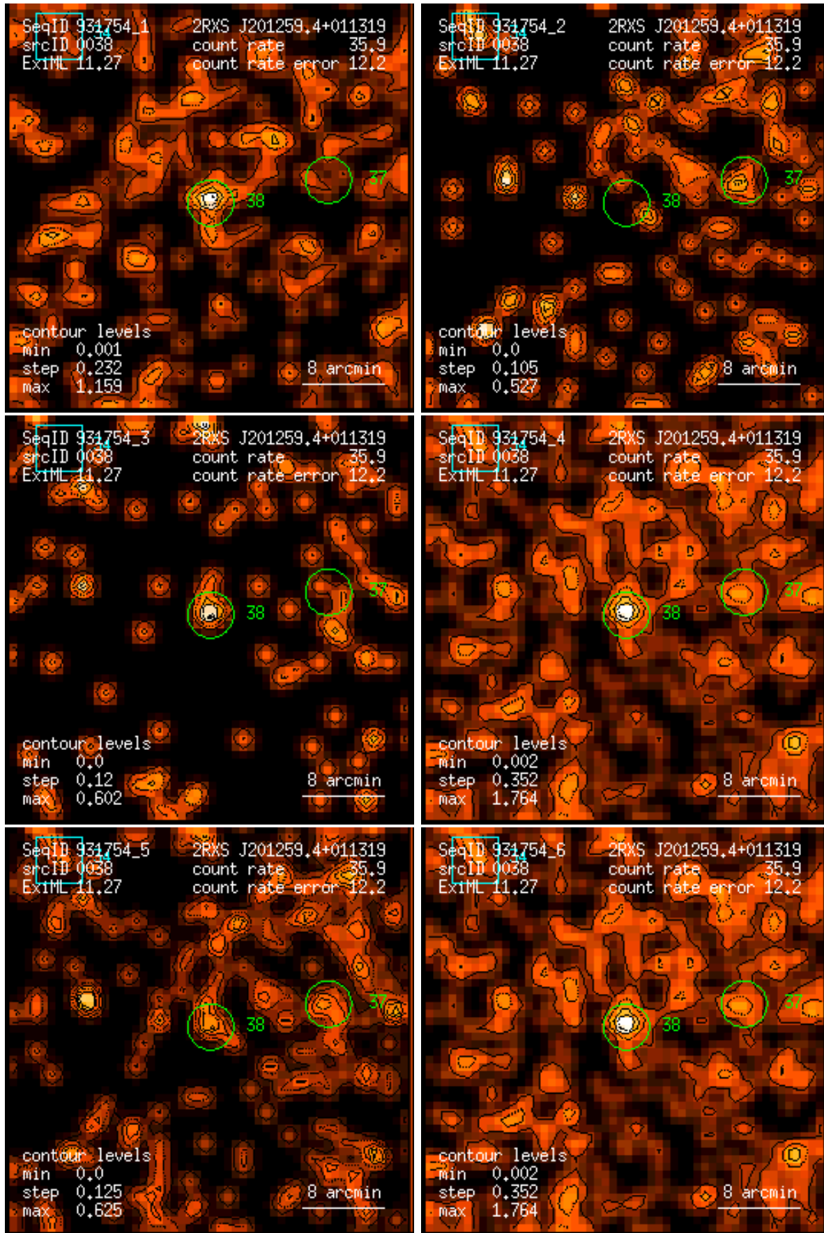
Figure 38: RASS 931754: detection 0038: band rate images, Gaussian filter: (1) PSPC channels 11 – 41, (2) 52 – 90, (3) 91 – 201, (4) 11 – 235, (5) 52 – 201, (6) 11 – 201. Broad band rates in counts/ks. Band rate contour levels in counts/ks/arcmin 2 .
